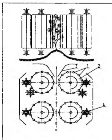
3.4-rasm. Seriyalab ishlab chiqarilayotgan VSh PTM apparati prinsipial sxemasi:
