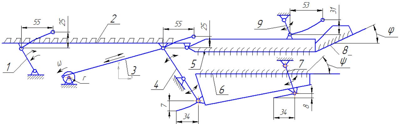
7.2-rasm. Tozalagichning kinematik sxemasi:
