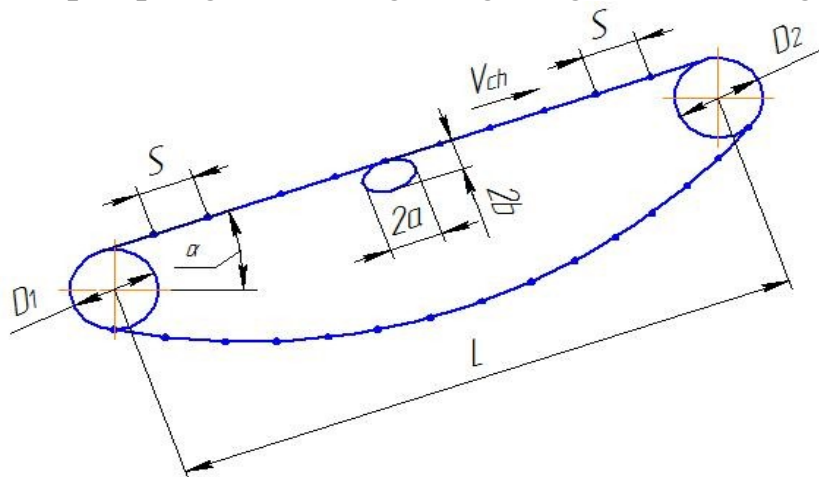
9.2-rasm. Chiviqli elevator sxemasi
