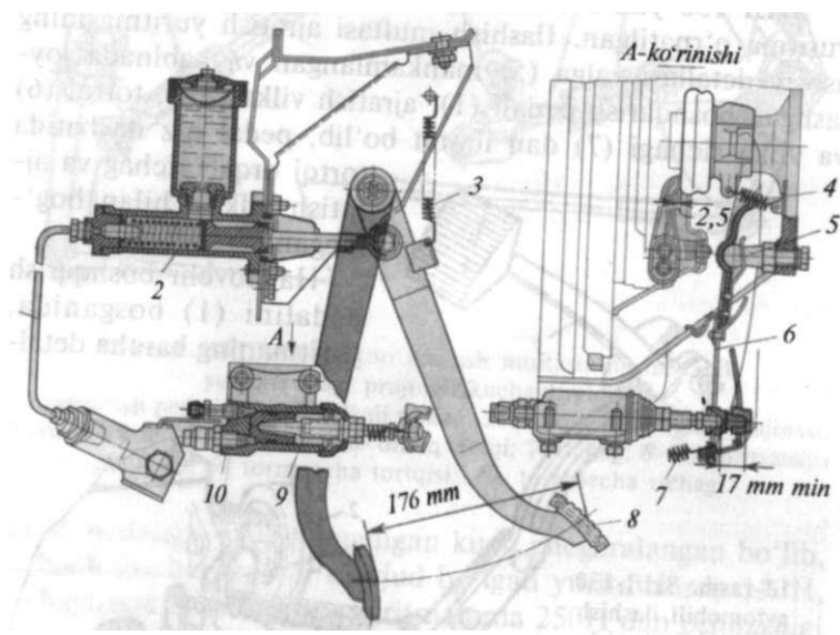
14-rasm. TA3-3102 avtomobili ilashish muftasini gidravlik boshqarish yuritmasi:
