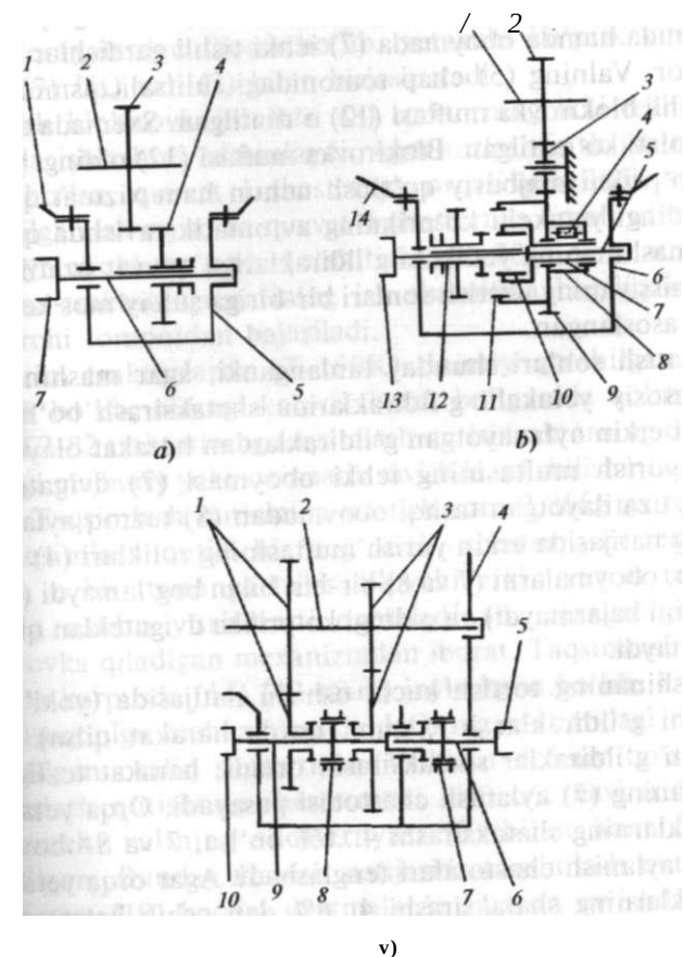
43-rasm. Taqsimlash qutilarining kinematik sxemalari:
