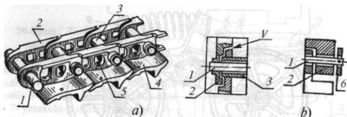
82-rasm. Himoyali va ochiq sharnirli zanjirlar: a — himoyali; b — ochiq; 1- barmoq; 2- zveno; 3- vtulka; 4- boshmoq; 5- bolt; 6- shayba; V — labirint.
