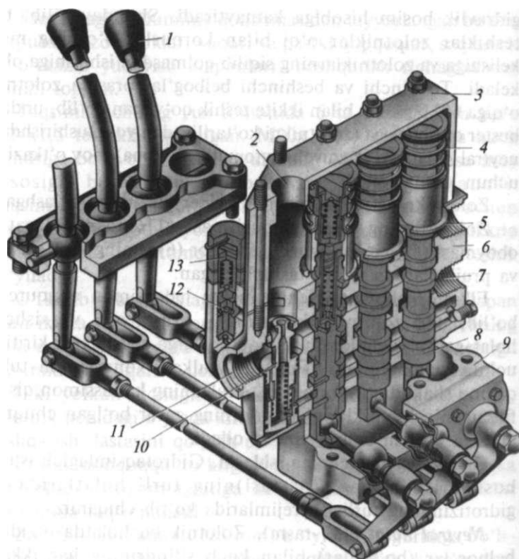
115-rasm. Gidrotaqsimlagich:
