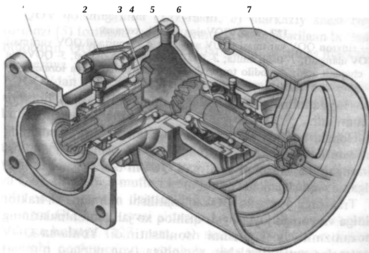
128-rasm. Yuritish shkivi.
