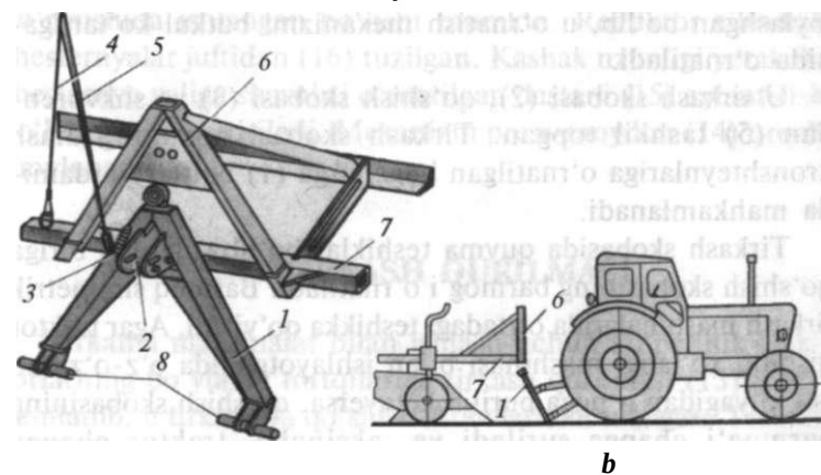
124-rasm. Avtotirkagich:
