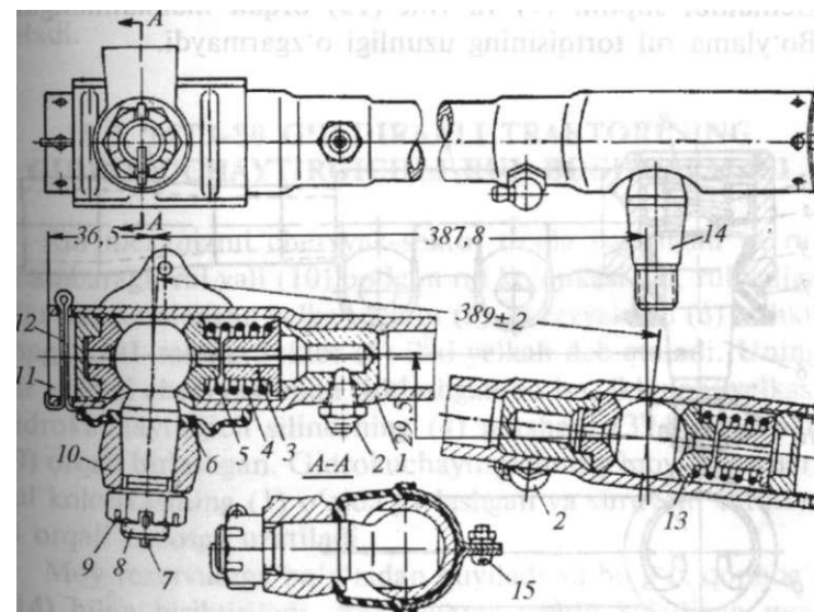
89-rasm. Bo'ylama rul tortqisi:
