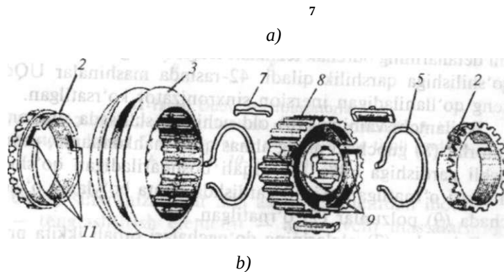
42-rasm. Inersion sinxronizator-
