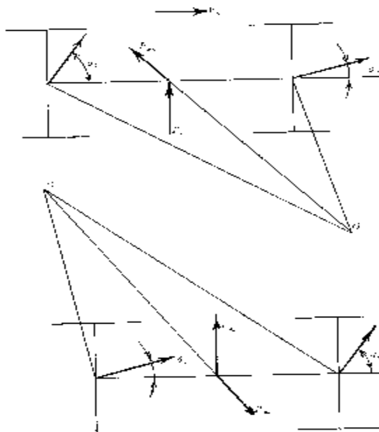
49-chizma. G'ildiraklarning yonaki sirpanish jarayonini o'rganishga oid shakllar.
