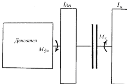
35-chizma. Traktor shig'ov bilan harakatlanishini o'rganishga doir ikki maxovikli dinamik model.
