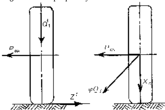
29-chizma. Shinaning yonaki sirpanish jarayoni.
