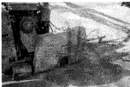
5.5-rasm. Qoplamadan nominal o'lchamdagi (15x15x60 sm) prizma namunani ajratib olish
