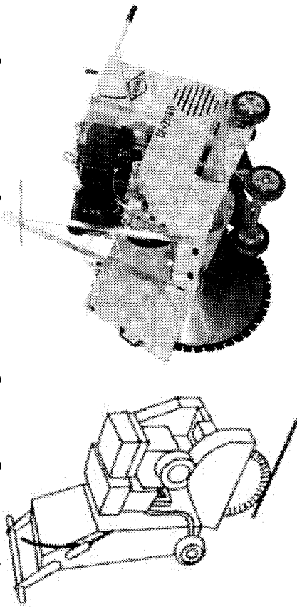
4.18-rasm. Deformatsiya choklari uchun olmos diskli chok kesgich
