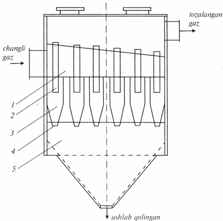
8.4- rasm. Batareyali siklonning tuzilishi:
