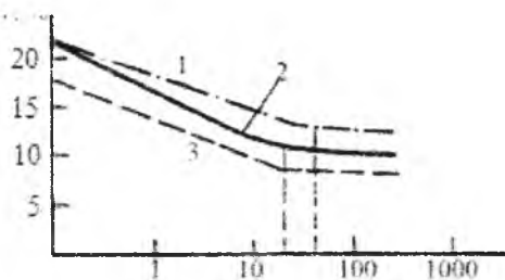
12-rasm. Grunt namligining unga bosim ta'sirining oshishiga qarab o'zgarishi: 1 – turli mineral tarkibli gillar; 2 – kaolinli gil; 3 – o'rtacha turli mineralli sug'lnok.
