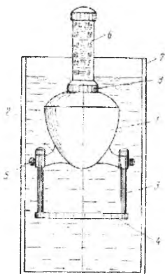
35-rasm. Gruntlarning suvda eruvchanligini aniqlash uchun PR asbobi: 1 – qalqib turuvchi metall; 2 – kronshteyn; 3 – oyoqcha; 4 – to'r; 5 – vint; 6 – trubka; 7 – idish; 8 – gayka.
