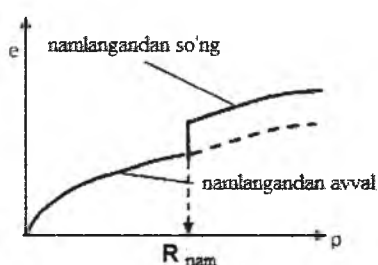
48-rasm. Lyossimon grunt-larning suv bilan namlagandagi kompression egri-si R_{nam} – namu-na namlanayotgan vaqtdagi yuk.
