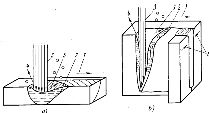
7.2-rasm. Elektron nurli payvandlashning sxematik ko'rinishi:
