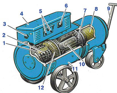
5.8-rasm. Payvandlash o'zgartirgichi:
