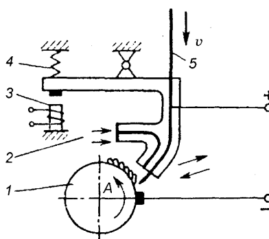
15.3-rasm. Vibro-yoy bilan eritib qoplash:
