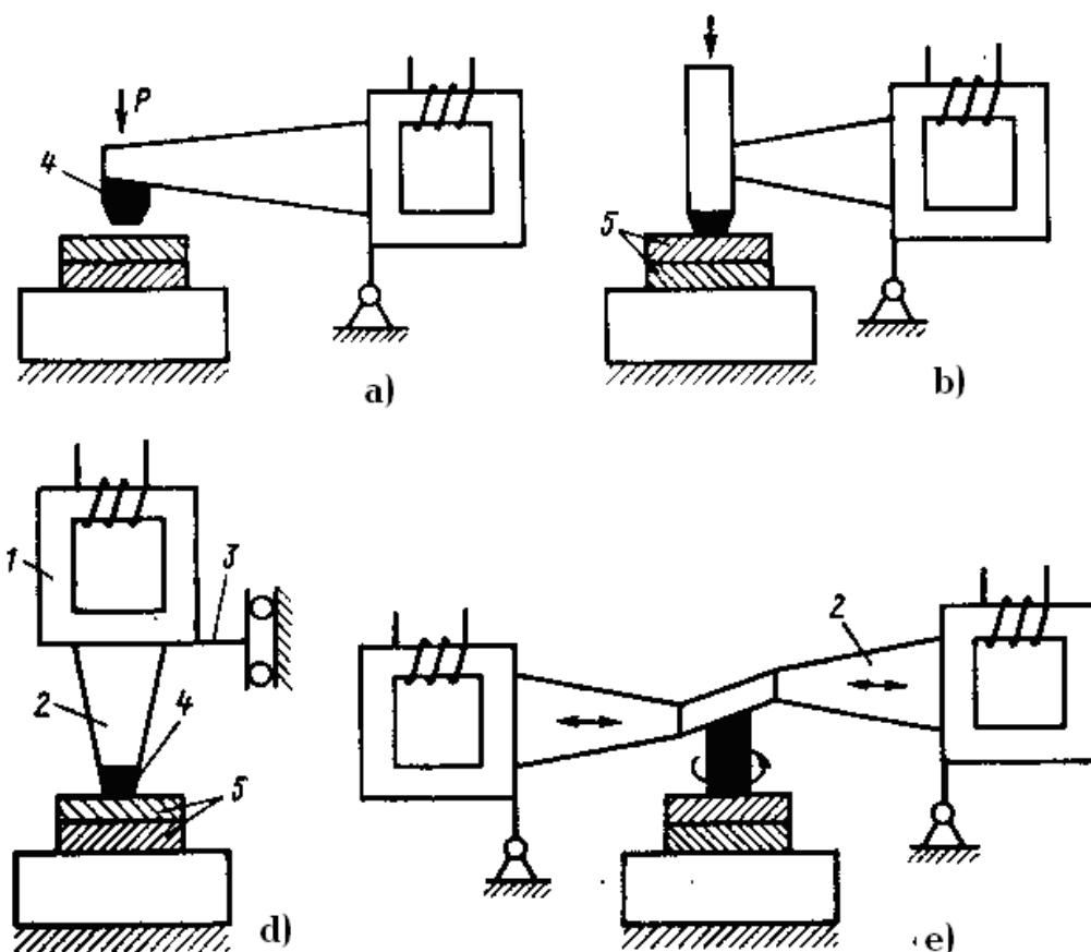
12.1-rasm. Ultratovush yordamida metallarni payvandlash uchun namunaviy tebranish tizimlari sxemasi:
