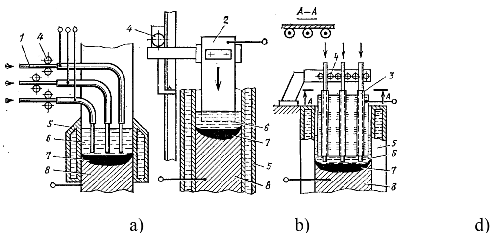
6.2-rasm. Elektr-shlak payvandlash usullari:
