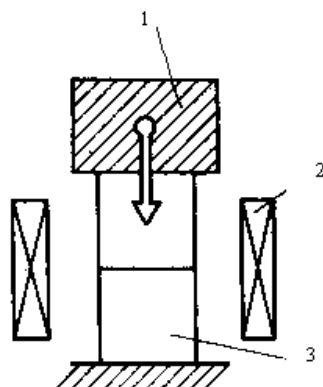
11.4-rasm. Erkin deformatsiyalash sxemasi bo'yicha diffuzion payvandlash:
