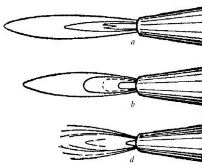
9.9-rasm. Payvandlash alangasining sxemalari:
