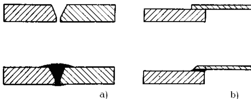
17.4-rasm. Kavsharlash-payvandlashda chok hosil bo'lish sxemasi:
