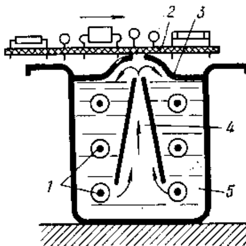
17.8-rasm. Eritilgan kavshar to‘lqini bilan kavsharlashning prinsipial sxemasi:
