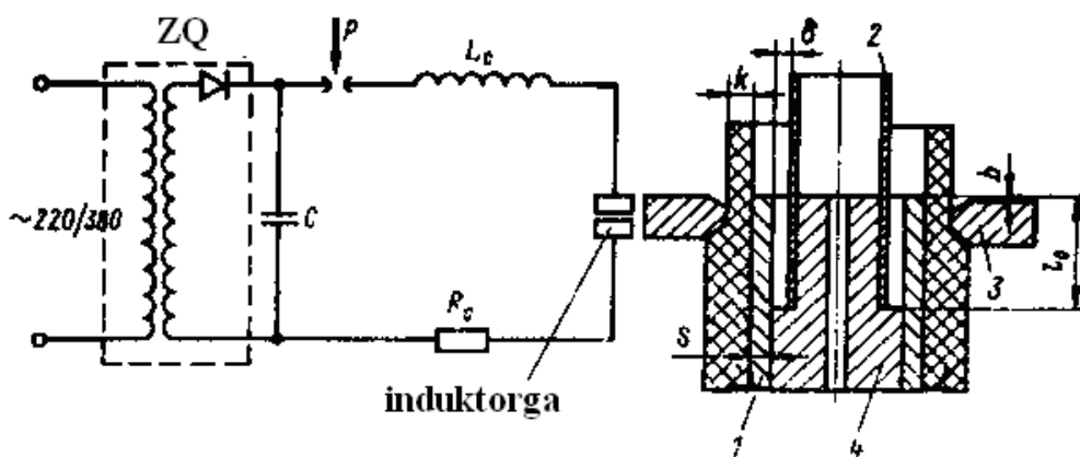
14.3-rasm. Magnit-impulsli payvandlash sxemasi:
