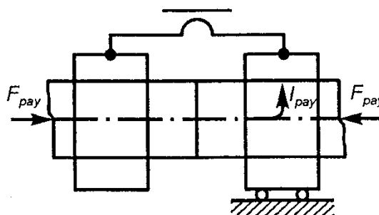
10.4-rasm. Uchma-uch payvandlash sxemasi.
