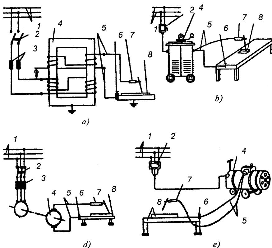
2.2-rasm. Yoy bilan dastakli payvandlash postining sxemasi:
