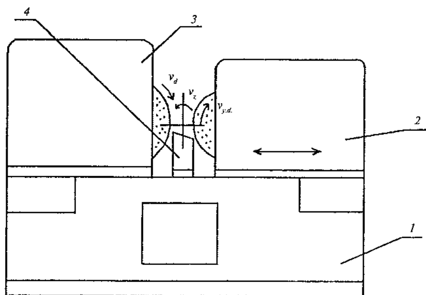
16.8- rasm. Markazsiz doiraviy jilvirlash stanogi. 1- stanina; 2-yetaklovchi doira babkasi; 3-jilviriash babkasi; 4-tayanch.
