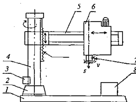
11.2- rasm. Radial- parmalash stanogi: 1-fundamentplitasi; 2-qo'zg'almas kolonna; 3-gidravlik qisqich; 4-buriluvchi gilza; 5-traversa; 6- rarmalash kallagi; 7-
