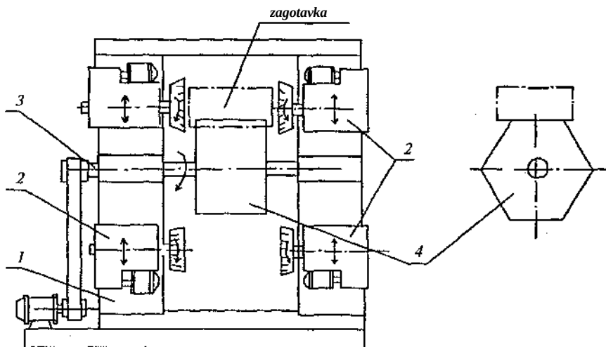
12.6-rasm. Barabanli frezalash stanogi: J-stoyka; 2-frezalash kallagi; 3-val; 4-baraban.
