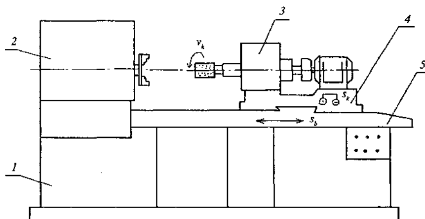
16.10-rasm. Ichki jilvirlash stanogi: 1-stanina; 2-mahsulot (old) babkasi; 3-jilvirlash babkasi; 4-karetk; 5-stol.
