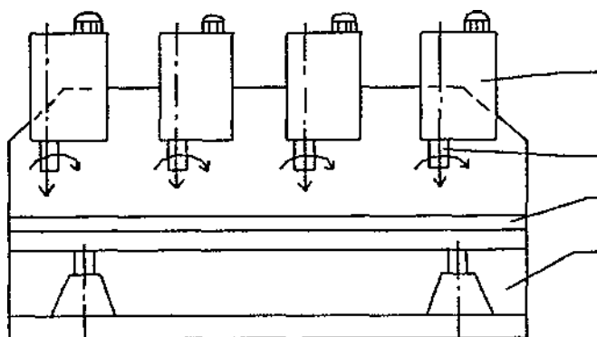
11.3-rasm. To'rt shpindelli vertikal-parmalash stanogi: 1- parmalash kallagi; 2-shpindel; 3-umumiy stol; 4-stanina.
