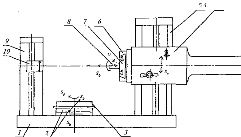
11.5-rasm. Teshik kengaytirish stanogi: 1-stanina; 2-salazkalar; 3-buriluvchi stol; 4-shpindel babkasi; 5-oldingi stoyka; 6-planshayba; 7-radial support; 8-shpindel; 9-orqa stoyka; 10-lyunet.
