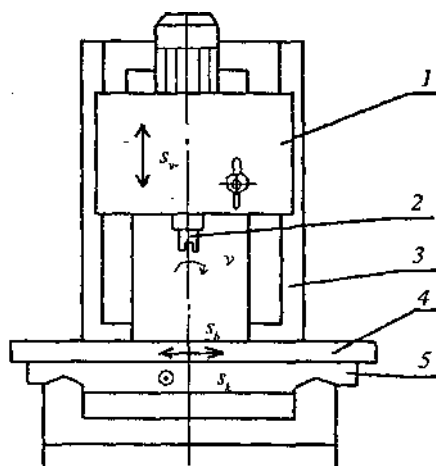
12.2- rasm. Krest stolli konsolsiz vertikal frezalash stanogi: 1-shpindel babkasi; 2-shpindel; 3- stanina; 4-stol; 5-karetko.
