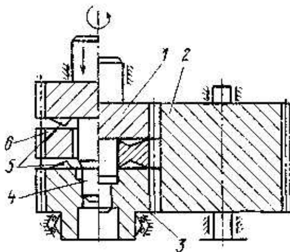
13.4.4-rasm. Tishli g'ildiraklarni plastik deformatsiyalash usulida tiklash
