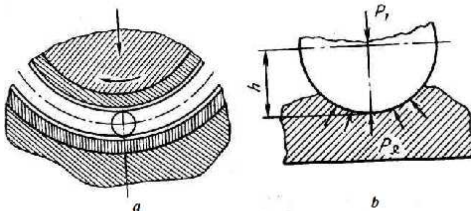
5.2.3 – rasm. Zoldirli podshipnikda kuchlar ta'sirining sxemasi:
