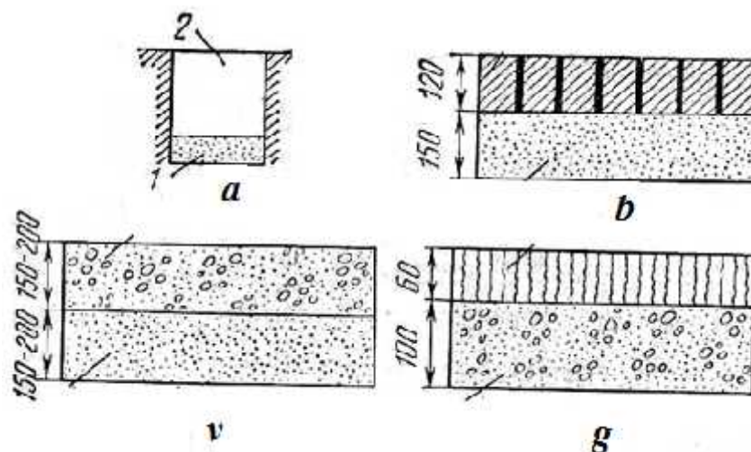
2.2.2-rasm. Mashina osti poydevori sxemasi
