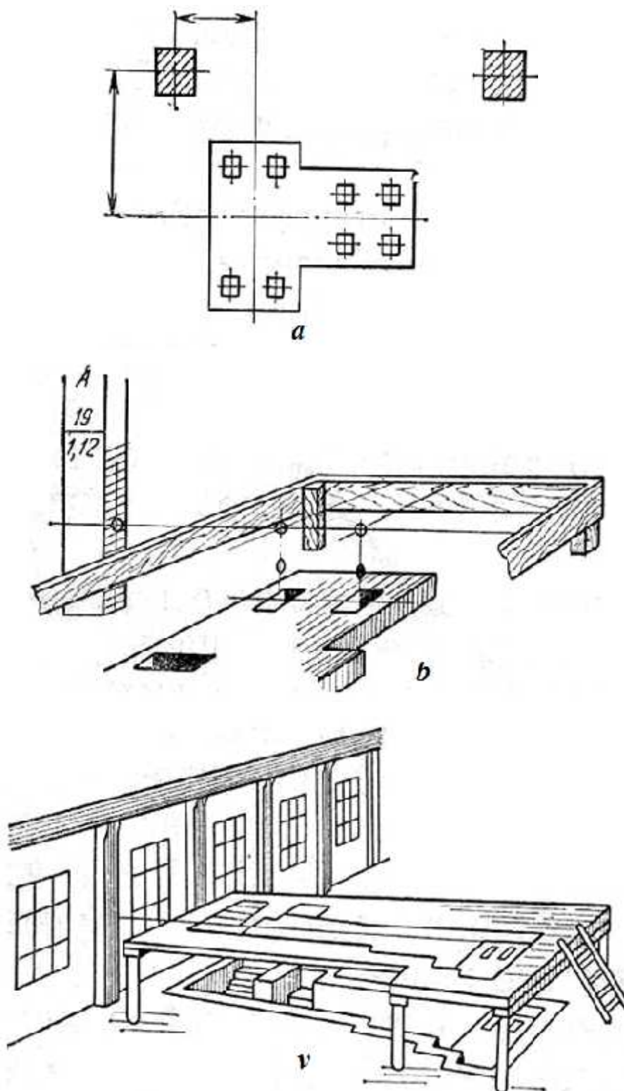
2.2.1-rasm. Mashinaning o'rnatilishi
