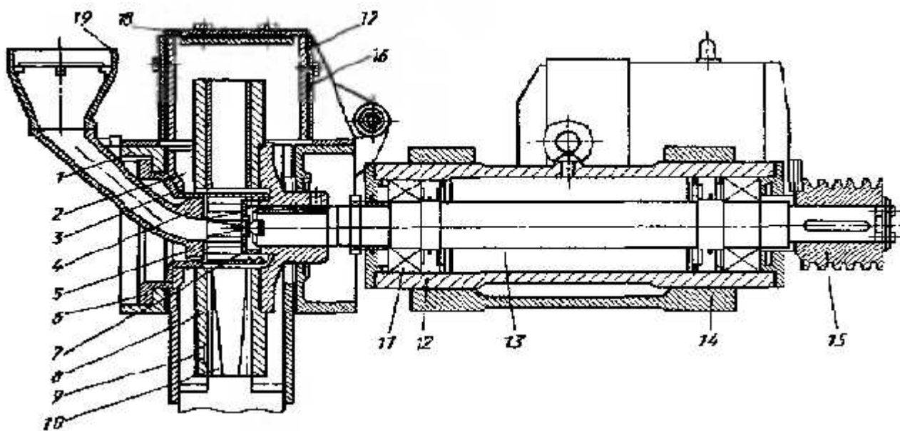
14.4.4-rasm. 2M393M markali pitra otish apparati:
