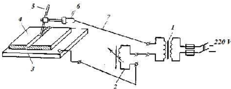
11.1.8-rasm. Elektr payvandlash apparatini ishga tushirish sxemasi
