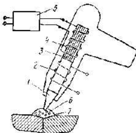
11.2.1-rasm. Ultratovushli kavsharlagich sxemasi.
