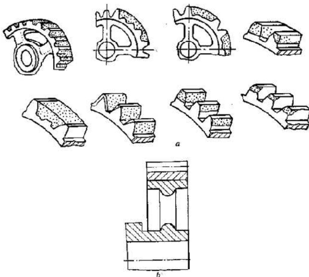
13.4.2-rasm. Tishli g'ildiraklarni tiklash usullari
