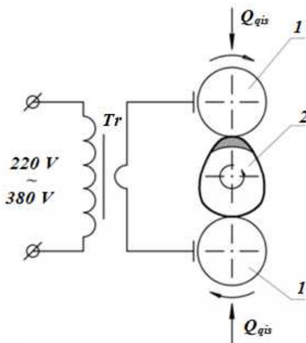
13.3.3-rasm. Payvandlab ulash sxemasi
