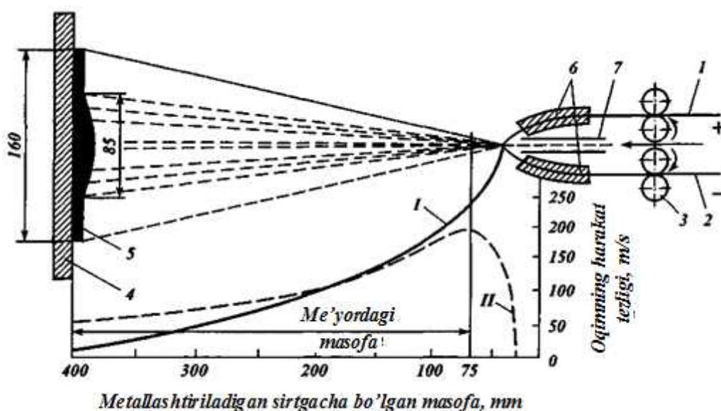
12.1.2-rasm. Elektr yoyli metallashtirish sxemasi:
