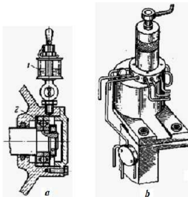
8.2.3-rasm. a – ignali moydon; b – nasos.
