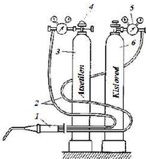
11.1.6-rasm. Gaz payvandlash qurilmasining sxemasi
