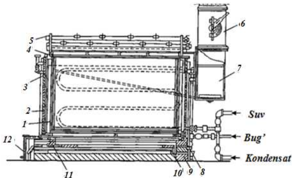
11.3.2-rasm. Galvanik usulda metall qoplash uchun vanna sxemasi:
