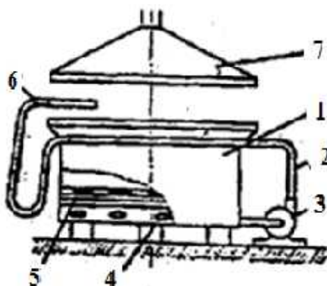
9.2.2-rasm. Issiq suv aralashmasi bilan yuvish vannasi.
