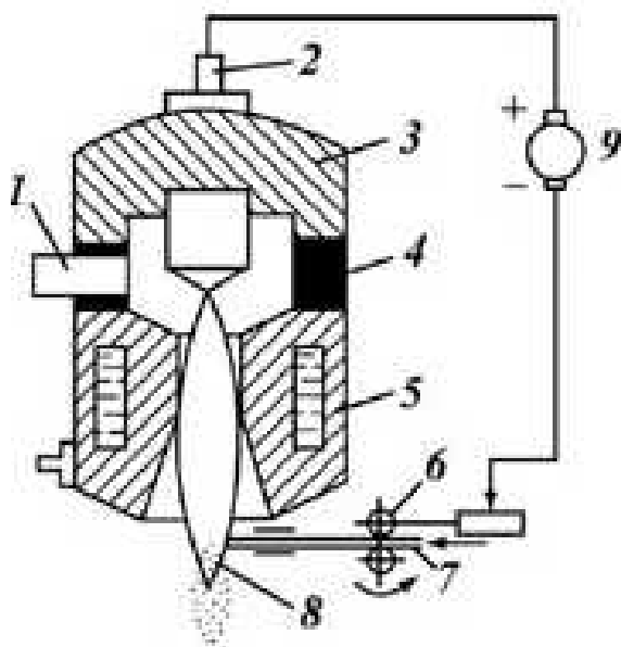
12.2.3-rasm. Sim bilan plazmali purkash sxemasi:
