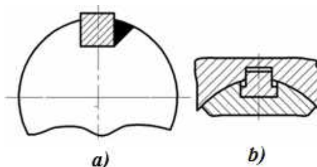
13.5.2-rasm. Shponka ariqchalarini ta'mirlash:
