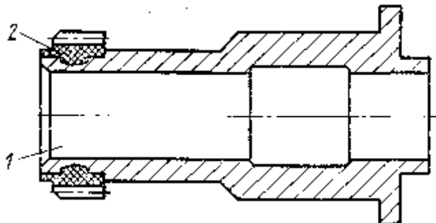
13.4.7-rasm. Polimer yordamida tiklanadigan tishli g'ildirak
