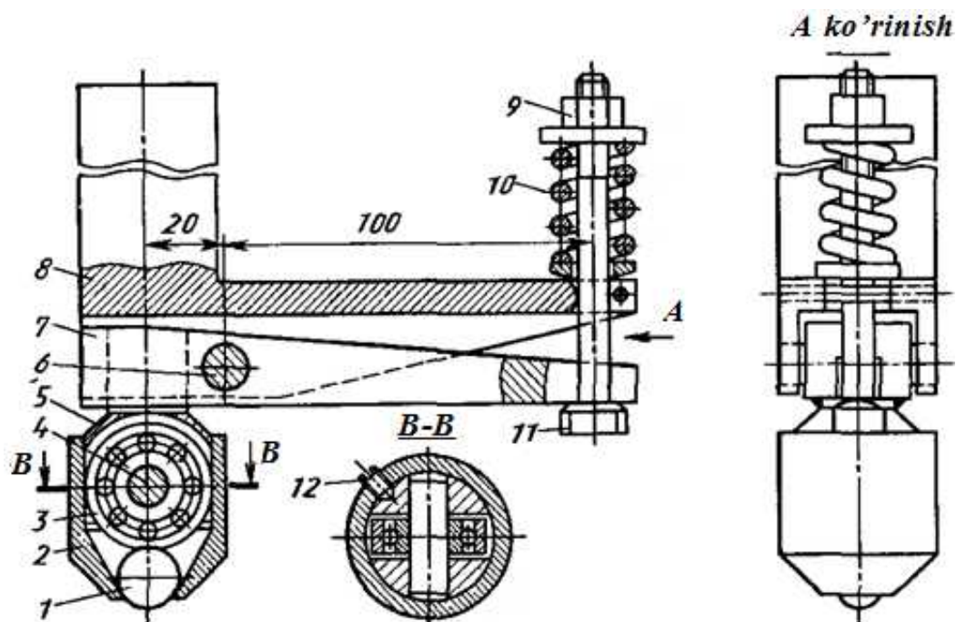
14.1.5-rasm. Randalash va karuselli stanoklarda prujina kuchini besh marta oshirish bilan detallarga ishlov berish uchun richagli harakatlanuvchi bir zoldirli dumalatgich:
