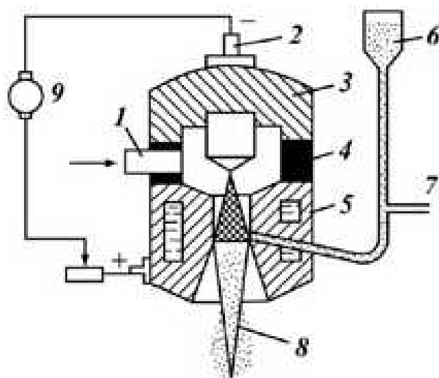
12.2.2-rasm. Kukun yordamida plazmali purkash sxemasi:
