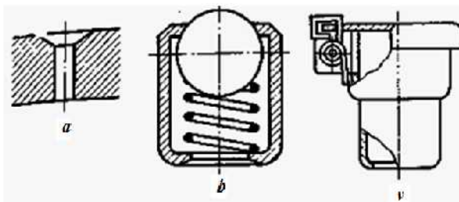
8.2.1-rasm. a – moylash teshigi; b – zoldirli moydon; v – qopqoqli moydon.
