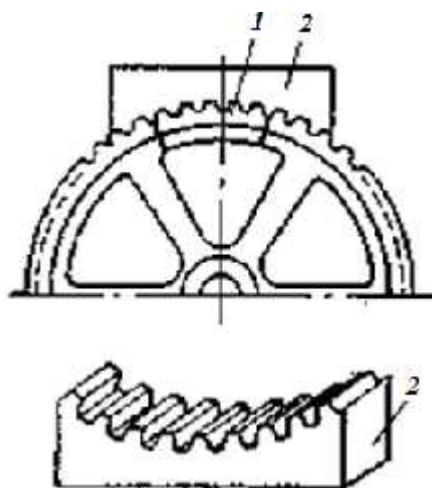
13.4.5-rasm. Tish qismlarini payvandlab ulash
