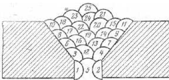
11.1.5-rasm. Payvandlash ketma-ketligi
