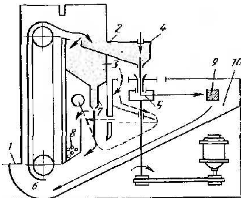
14.4.5- rasm. DU-1 markali pitra otish qurilmasining sxemasi:
