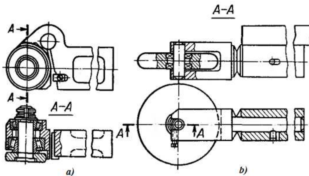
14.2.8-rasm. Detal sirtiga 30000 N gacha kuch bilan ishlov berish uchun maxsus dumalatish qurilmasi:
