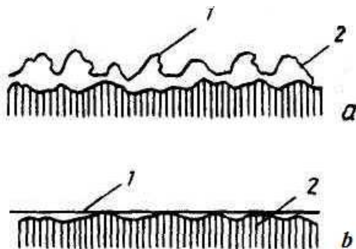
5.2.2-rasm. Siyqalanish jarayonida detal sirtidagi notekisliklarning o'zgarishi:
