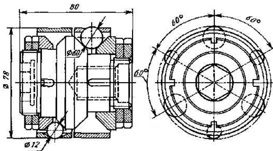
14.1.10-rasm. Qattiq ikki qatorli dumalatgich.
