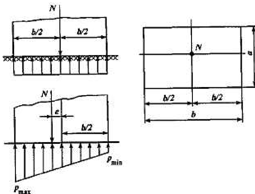
2.2.4-rasm. Bosimning tuproqqa taqsimlanishi.
