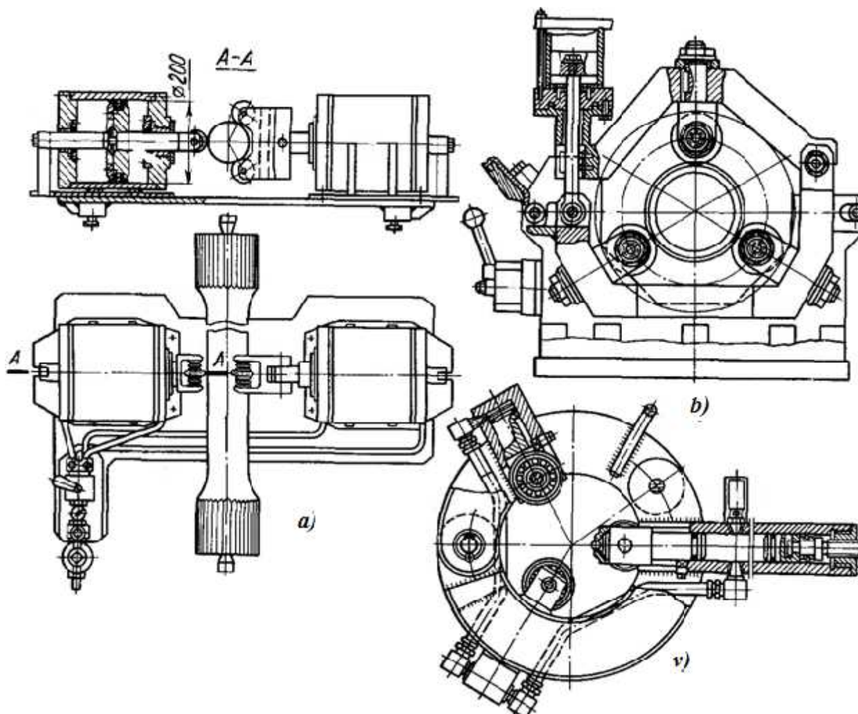
14.2.10-rasm. Uch rolikli moslamalar:
