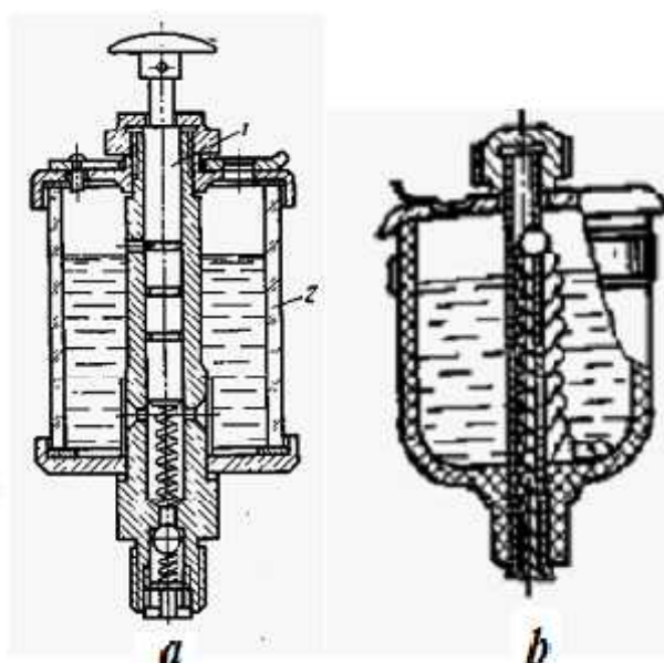
8.2.2-rasm. a – plunjerli nasos; b – pillikli moydon.
