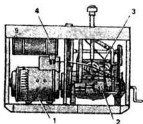
5.9 - rasm. Payvandlash agregati:
