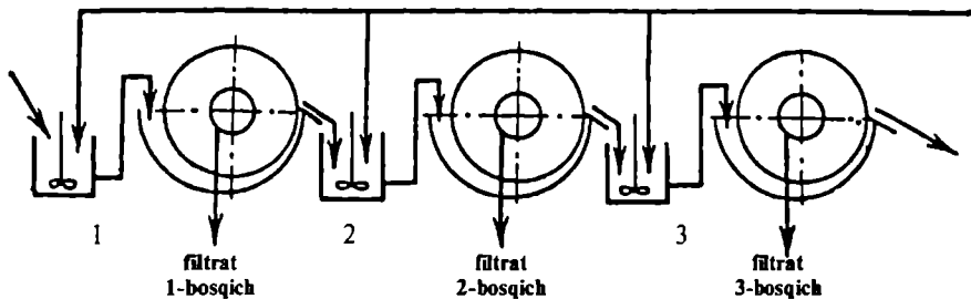
15-rasm. Cho'kmani uch bosqichda ketma-ket yuvish sxemasi: 1-3 repulpatorlar.
