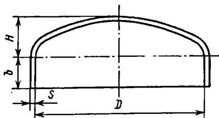
93-rasm. Ellipssimon tub
