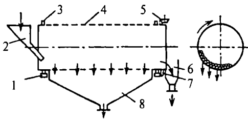
27-rasm. Barabanli g'alvir mashina sxemasi:
