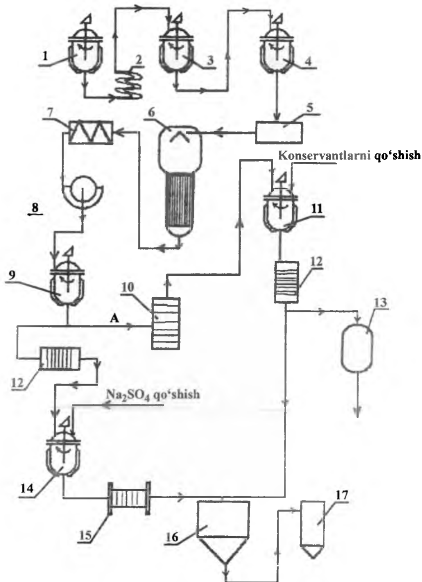
17-rasm. Ferment olinishining taxminiy texnologik sxemasi:
