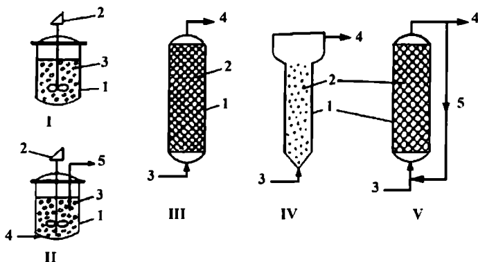
18-rasm. Fermentni immobillovchi bioreaktor:
