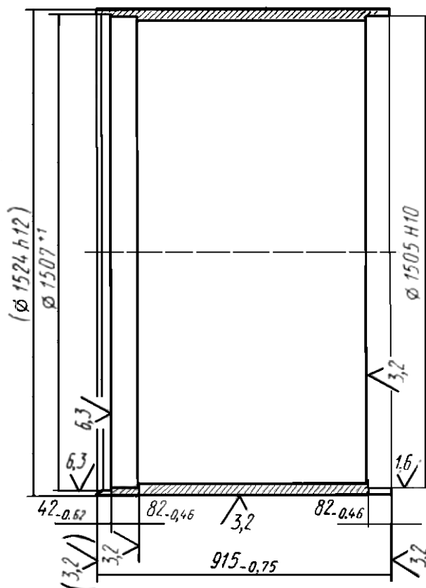
7.2-rasm. Pulatdan kilingan bosh barabandagi obechayka.
