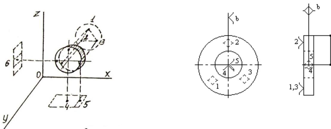
2.17 – rasm. Disk detallarni asoslash.
