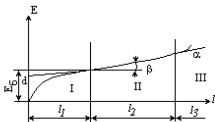
2.7- rasm. Eyilishni egri chizig'i
