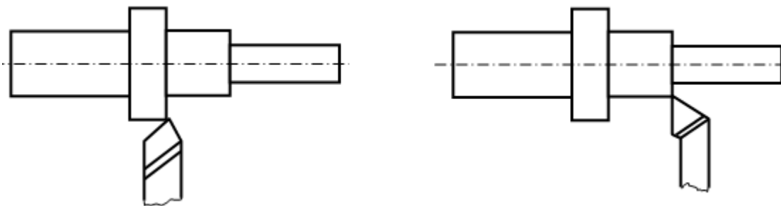
5.2-rasm. Yuzalarga navbatma-navbat ishlov berish
