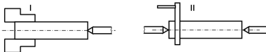
5.5-rasm. 5.5-rasm. Ishlov berish uchunssilindrik valikni tokarlik dastgoxiga maxkamlash usullari
