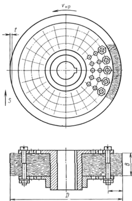
10.2-rasm. Metall cho'tka
