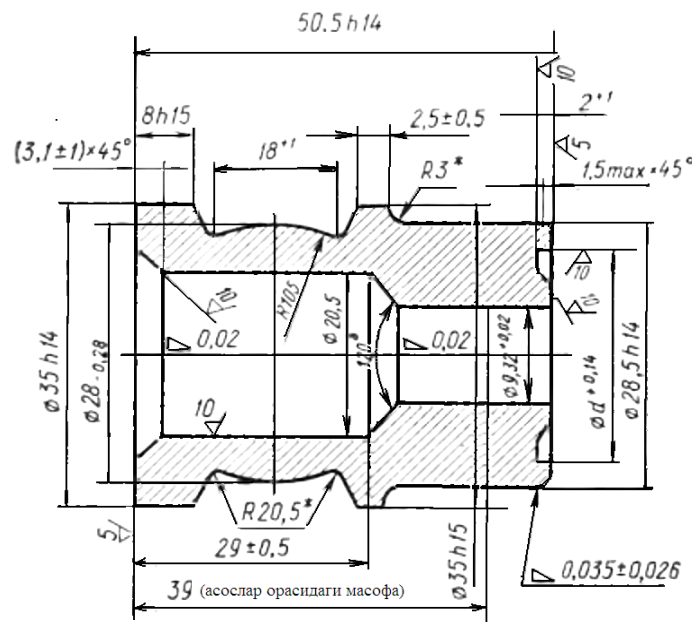
8.5-rasm. Urchuq dumaloqchasi
