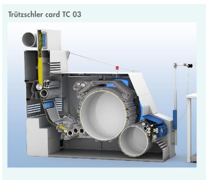
1.5-rasm. Tarash dastgohining ko'ndalang qirqim ko'rinishi.
