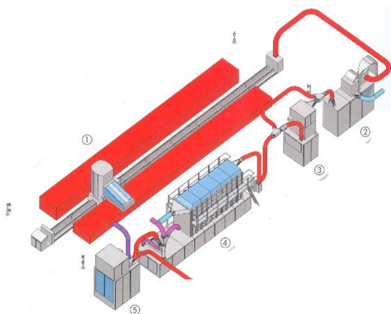
1.2-rasm. Truetzschler firmasining universal titish-tozalash agregati.
