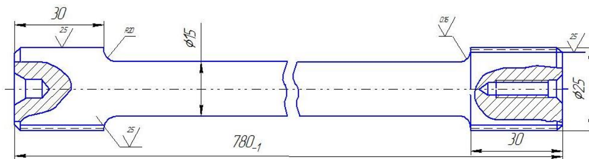
9.1-rasm. Torsion val
