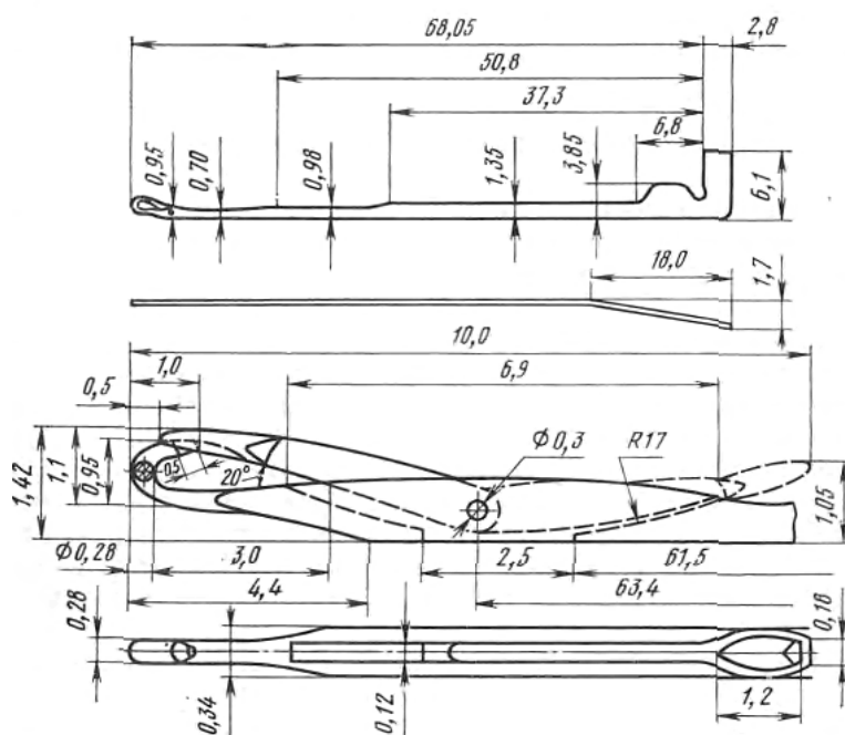
10.3-rasm. Trikotaj mashinasini ignali tilchasi
