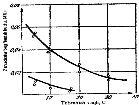
15.6-rasm. Gruntidagi bog'lanish kuchining vaqt davomida o'zgarishi
