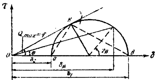
5.2-rasm. Sochiluvchan gruntning siljishiga oid Moor diagrammasi.
