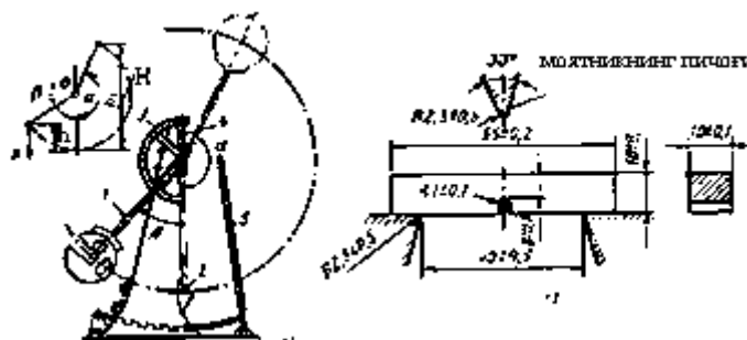
6.9-rasm. Mayatnikli kopyor
