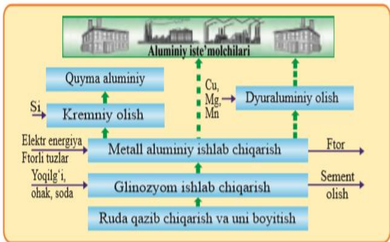
7-rasm. Aluminiy ishlab chiqarish
