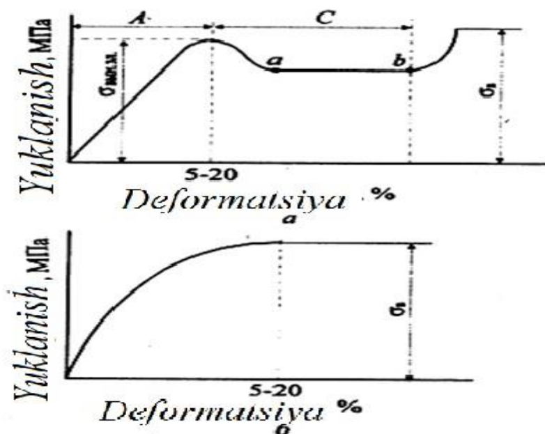
16.8-rasm. Cho'zish diagrammasi:
