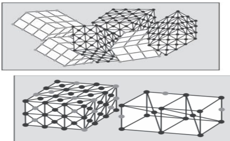
5.2-rasm. Kristallanish darajasi.
