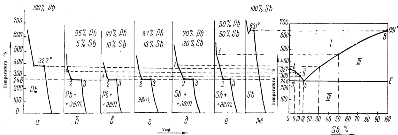
5.5-rasm . Qo'rg'oshin – surma qotishmalarining sovish egri chiziqlari (chapda) va holat diagrammasi (o'ngda)
