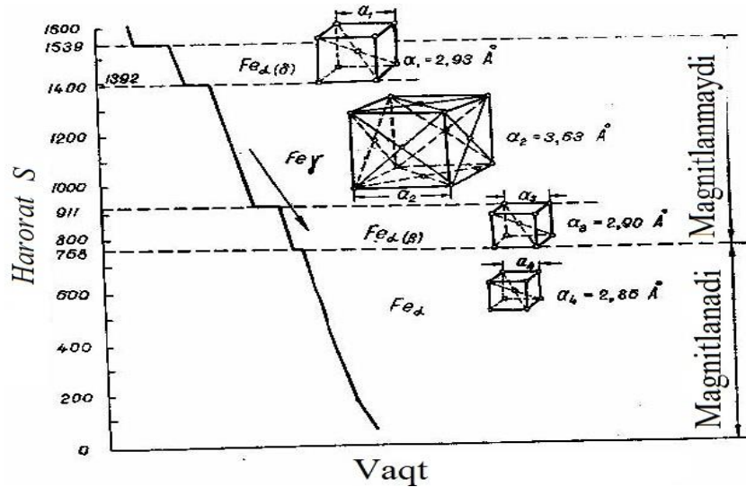
4.11-rasm. Haroratga qarab temirning kristallanishi
