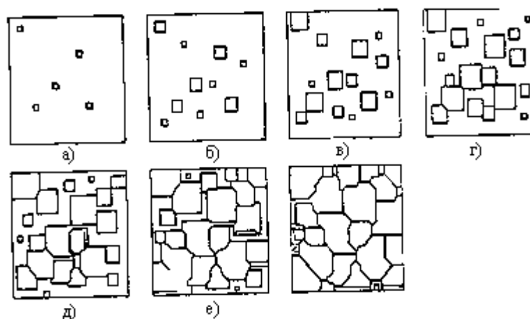
6.11-rasm. Metallarning kristallanish jarayonining sxemasi
