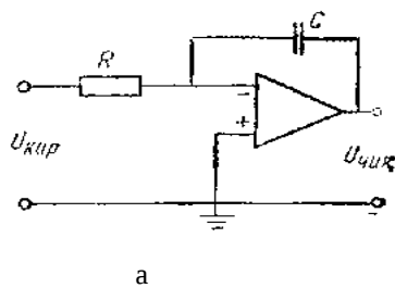
5.10 –rasm. Kirish signalini integrallovchi (a) va differensiallovchi (b) kuchaytirgich sxemalari
