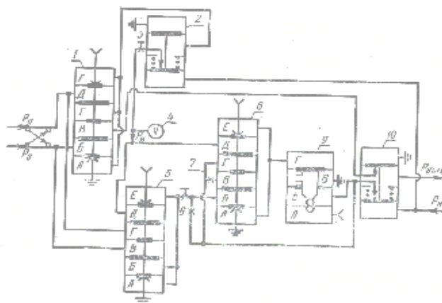
8.2-rasm. Proporsional-integral rostlagichning prinsipial sxemasi.
