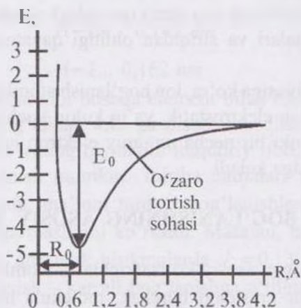
4.1-rasm. Ikki atomli molekula potensial energiyasining o'zgarishi.
