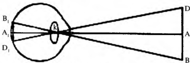
24-rasm. Nurlarning ko'z gavharida sinishi:
