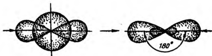
( s + p )- orbital
