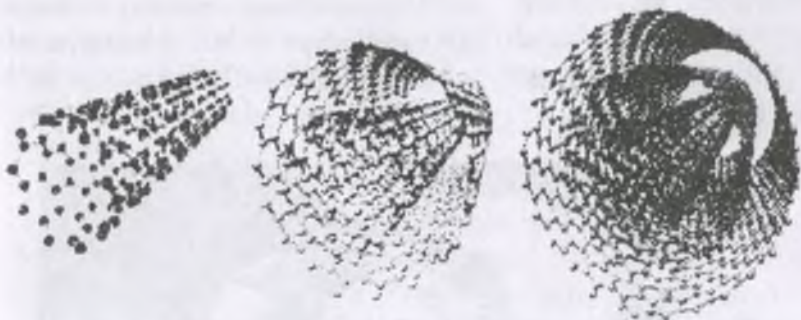
42-rasm. Nanotrubkalar
