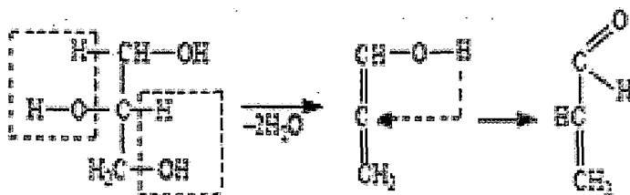
akrolein
