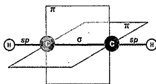
25-rasm. Asetilen molekulasida \sigma -bog'lanish(A) va \pi -bog'lanish(B)ning hosil bo'lishi.
