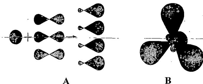
20-rasm. Uglerod atomining sp^3 -gibridlanishi (A) va modeli (B).
