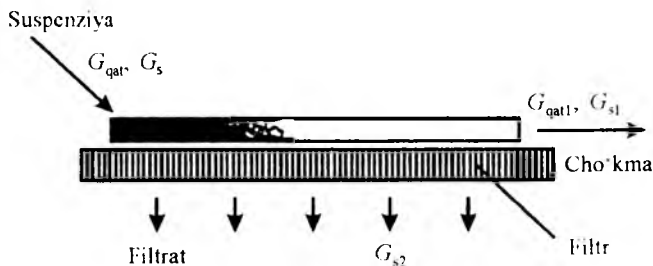
5.13-rasm. Suspensiyani ajratish uchun filtr.
