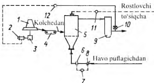
4.25-rasm. Kolchedanni kuydirish uchun qabul qilish pechini rostlovchi avtomatik sxema: 1–tarekchasimon ta'minlagich; 2–ta'minlagich yuritmasi; 3–reduktor; 4 – oraliq transporter; 5–pech; 6–diafragma; 7, 11, 12–rostlagichlar; 8 – rostlovchi to'sma qopqoq; 9–qozon-utilizator; 10–gazanalizator (SO 2 uchun).
