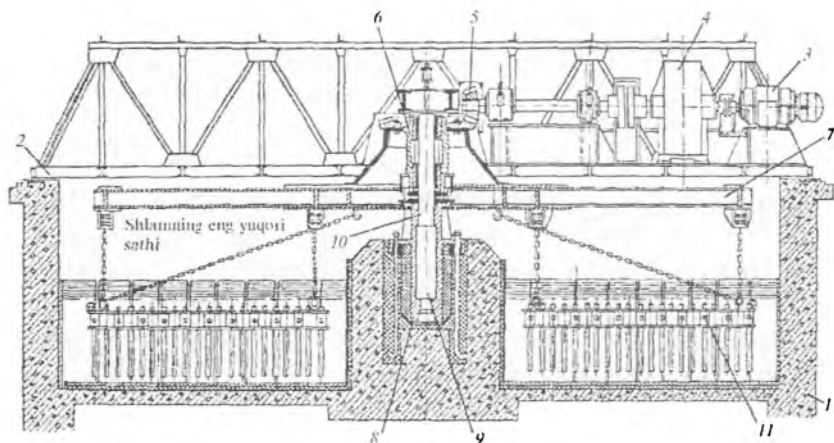
8-rasm. Loychayqatgich.
