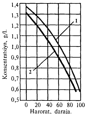
7-rasm. \text{Ca(OH)}_2 va \text{CaO} larning haroratga qarab eruvchanligi:
