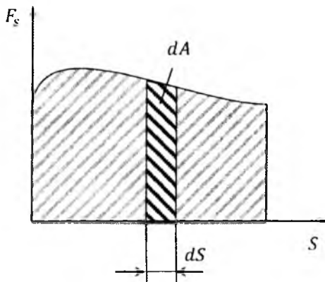
4.2-rasm. To'g'ri chiziqli harakatda bajarilgan ishning geometrik tasviri
