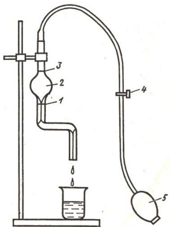
12-rasm Stalagmometr.
