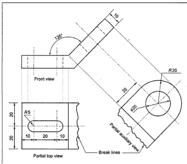
Figure 13.6 Partial Views
