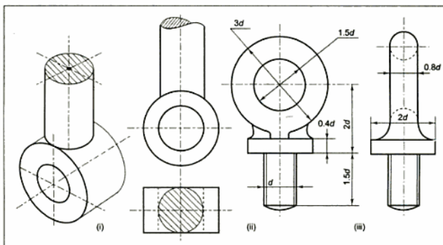
Figure 17.34 Eye Bolts
