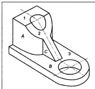
Figure S.15.10(b) Solution
