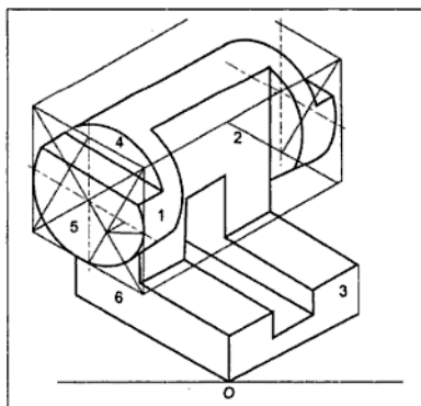
Figure S.15.12(b) Solution
