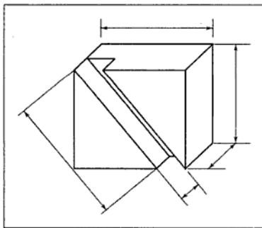
Figure 12.19 Dimensioning Oblique Parallel Projection
