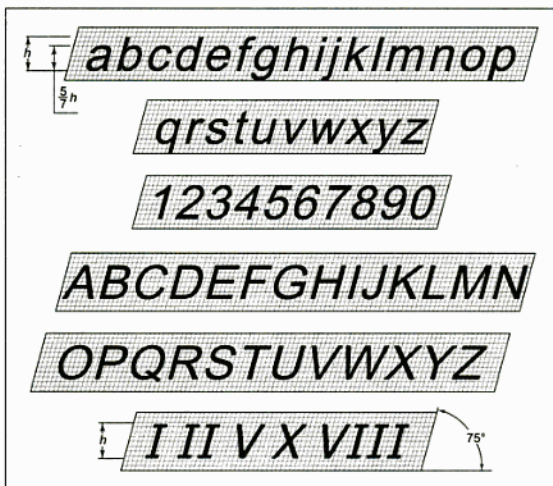
Figure 1.14 Sloping Letters
