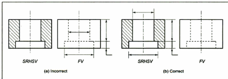
Figure 12.10 Take Dimensions from Visible Outlines
