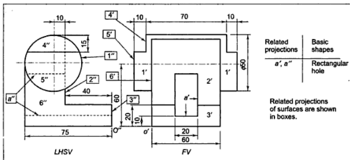
Figure S.15.12(a) Relations of Surfaces and of Basic Shape
