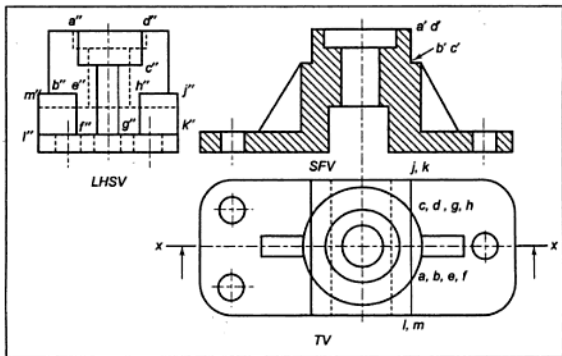
Figure S.14.9 Solution
