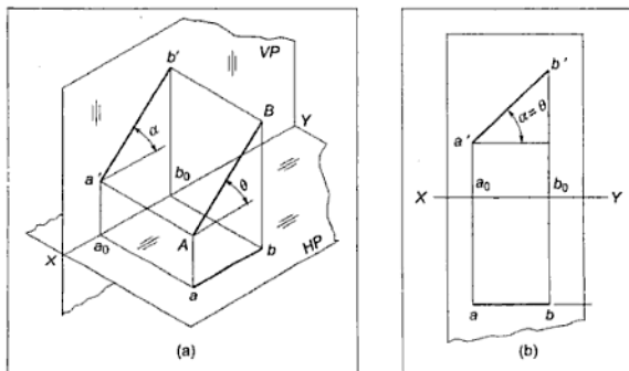
Figure 3.10 Line Parallel to the VP and Inclined to the HP
