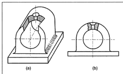
Figure 11.15 Partial or Broken Section
