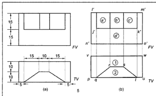
Figure 14.23 Locating Projections of Plane Surfaces in Other Views
