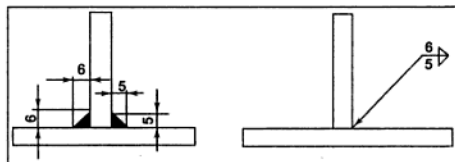
Figure 18.16 Indication of Size of Weld
