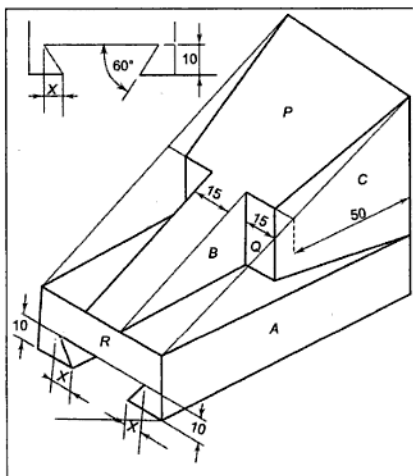
Figure S.15.5(b) Solution
