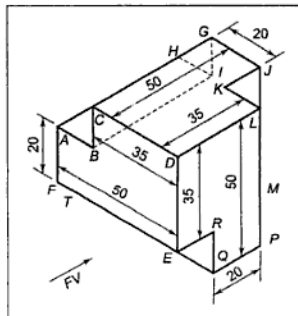
Figure 10.26 Object with Coinciding Lines in Pictorial View
