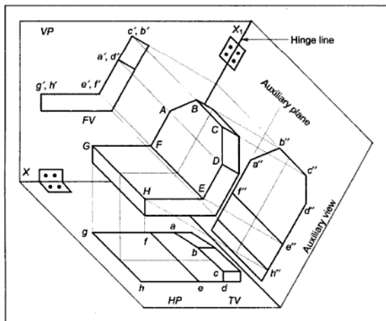
Figure 13.1 Projection of an Auxiliary View on an Auxiliary Plane of Projection
