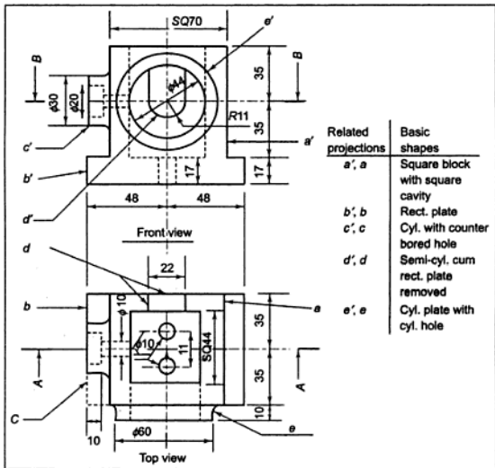
Figure S.14.10(a) Basic Shape Relations
