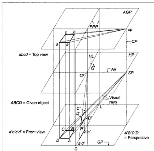
Figure 16.15 Terminology of Perspective Projection
