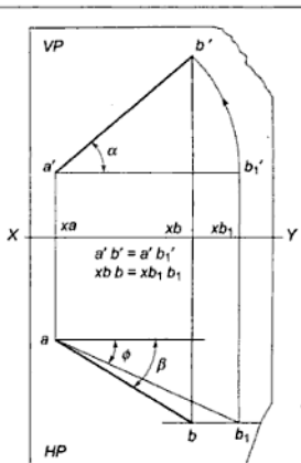
Figure 3.22(b) Projections of Lines Inclined to Both HP and VP
