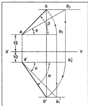
Figure 3.26 Example 3.6 (III Angle)
