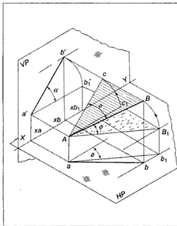
Figure 3.22(a) Lines Inclined to Both HP and VP
