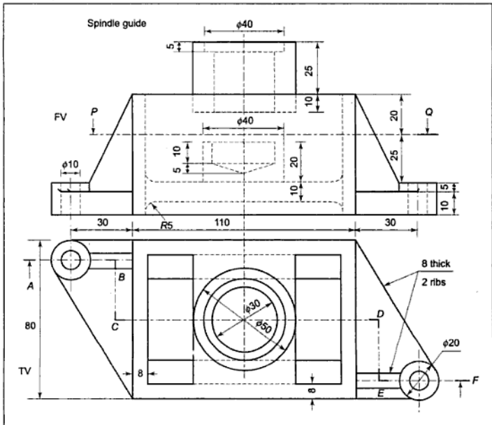
Figure 14.31(a) Example 14.7
