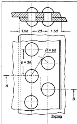
Figure 18.7 Double Riveted Zigzag Lap Joint
