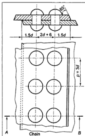
Figure 18.6 Double Riveted Chain Type Lap Joint
