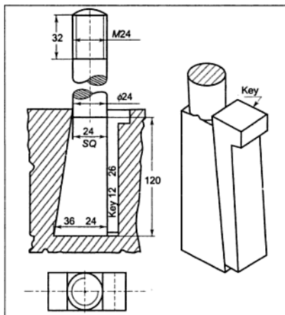
Figure 17.43 Lewis Foundation Bolt
