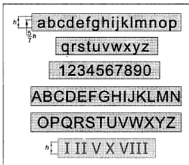
Figure 1.13 Vertical Letters
