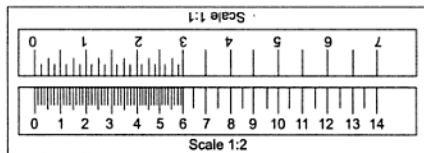
Figure 1.7 Scales
