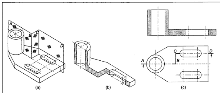
Figure 11.12 Offset Section
