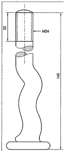
Figure 17.39 Twisted Foundation Bolt
