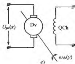
2.20-rasm. RC zanjiri (a); LR zanjiri (b); o'zgarmas tok generatori (d); o'zgarmas tok dvigateli (e).
