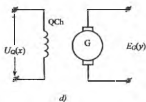
2.20-rasm. RC zanjiri (a); LR zanjiri (b); o'zgarmas tok generatori (d); o'zgarmas tok dvigateli (e).
