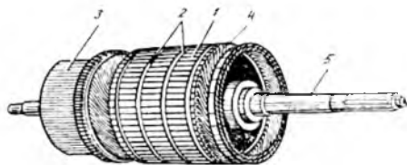
27.2-rasm. (O'zgarmas tok mashinasining yakori: 1 – yakor o'zagi; 2 – bandajlar; 3 – kollektor; 4 – yakor chulg'aminging pazlardan tashqari qismi; 5 – val.
