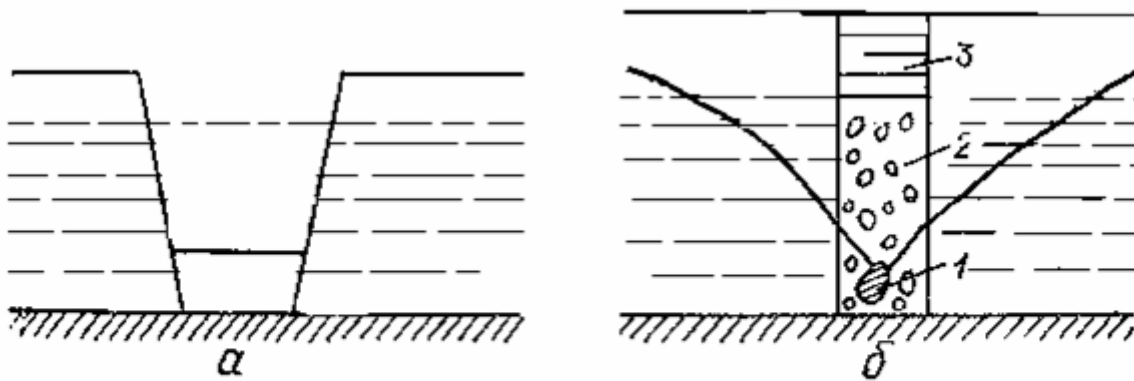
7.18-rasm. Gorizontall drenlar. a-ochiq handaq, b-yopiq handaq 1-handaq quvuri, 2-filtrlovchi material, 3-filtrlovchi materiali saqllovchi gilli grunt qatlami
