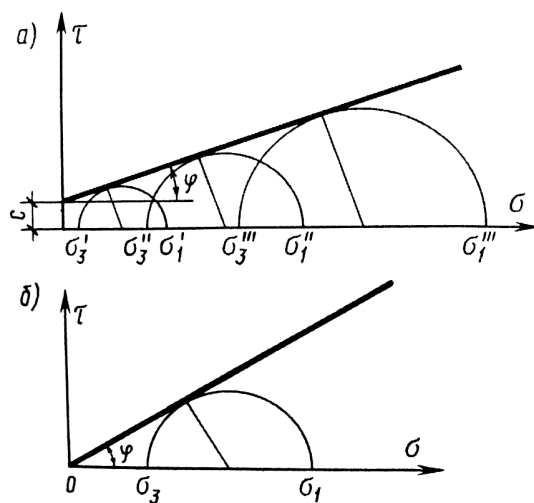
2.13-rasm. Stabilometrdagi sinov-lar bo'yicha gruntning mustahkamlik ko'rsatkichlarini aniqlash: a – bog'lanishli grunt; b – sochiluvchan grunt
