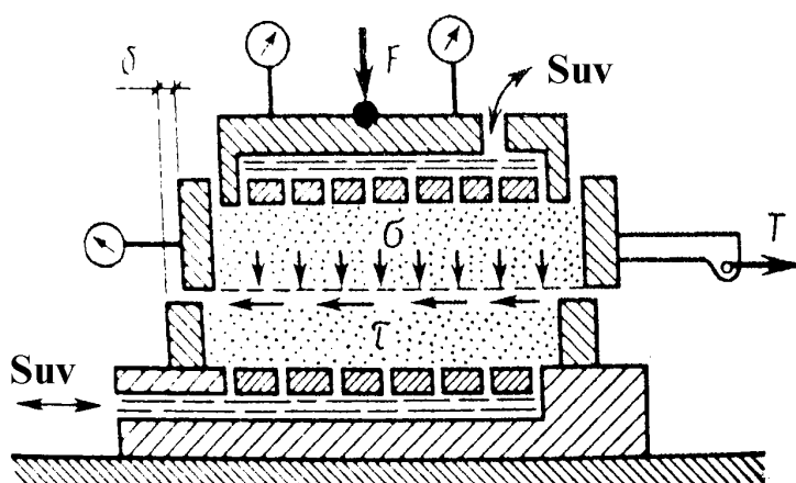
2.9-rasm. Siljish asbobi sxemasi
