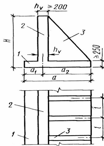
6.12-rasm. Qovurg'ali burchaksimon tirkak devor:
