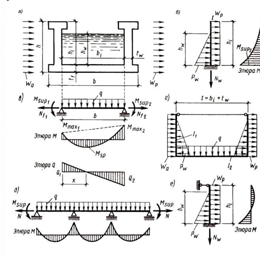
3.6-rasm. Inshoot novining ko'ndalang yo'nalish bo'yicha hisoblash sxemalari
