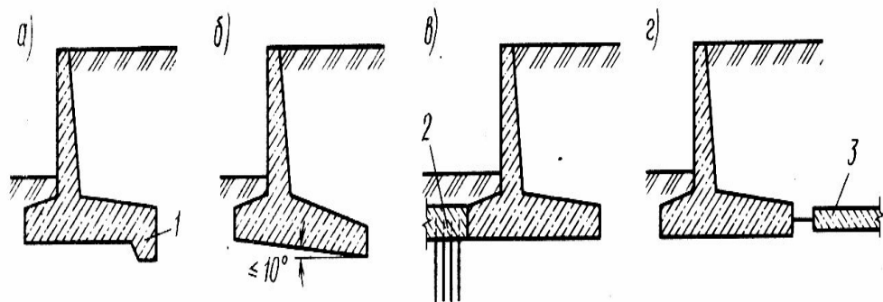
6.3-rasm. Tirgak devorlarning ustivorligini oshirish usullari
