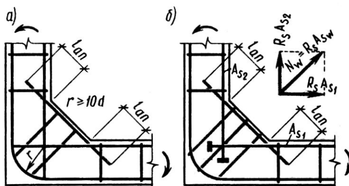
4.4-rasm. G – shaklidagi tugunlarning kirish burchagidagi cho'zilgan qirralarini aramturalash
