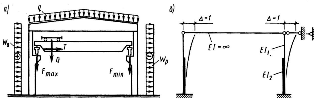
1.18-rasm. Bino ko'ndalang ramalarini hisoblash sxemalari
