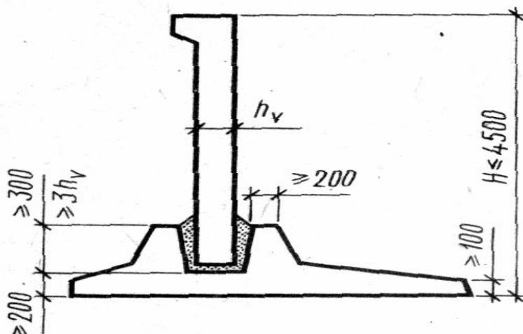
6.6-rasm. Burchaksimon yig'ma temirbeton tirgak devor
