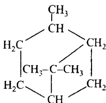
pinan
