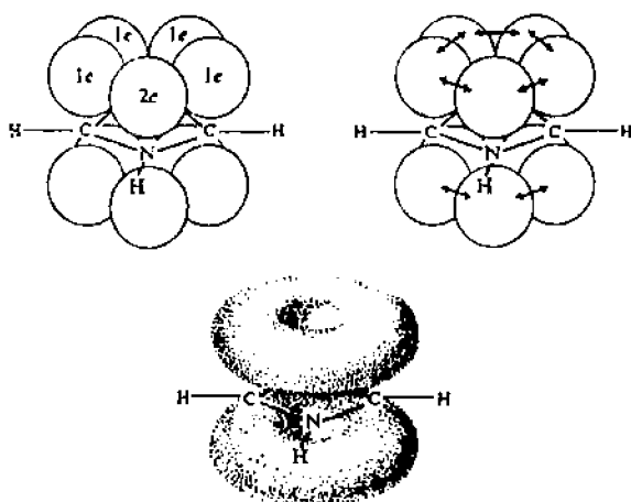
4-rasm. Pirrolning tuzilishi.
