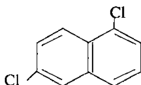
epi – dixlor- naftalin
