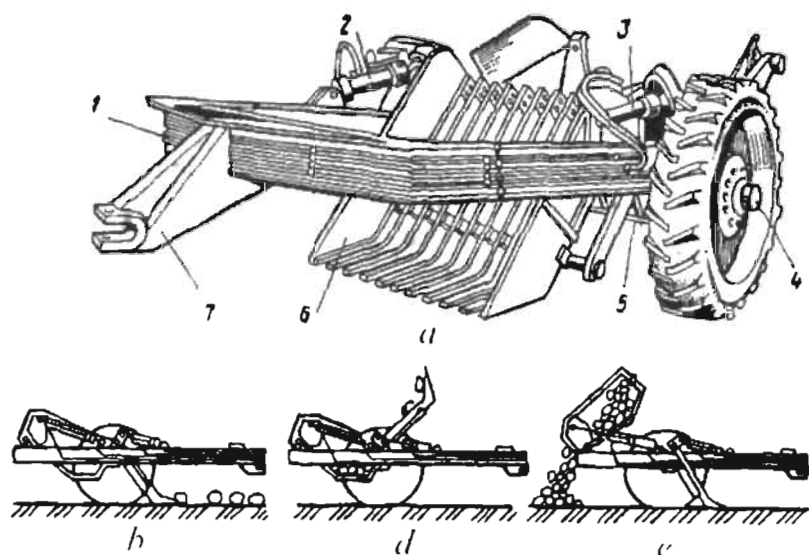
3.1.13-rasm. UKP-O6 markali tosh terish mashinasi:
