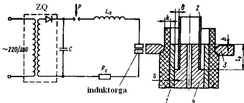
14.3-rasm. Magnit-impulsli payvandlash sxemasi:
