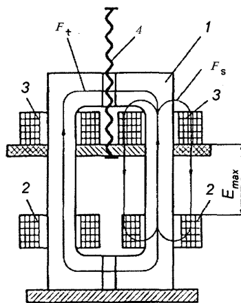
5.2-rasm. Suriladigan cho‘lg‘amli payvandlash transformatorining chizmasi:
