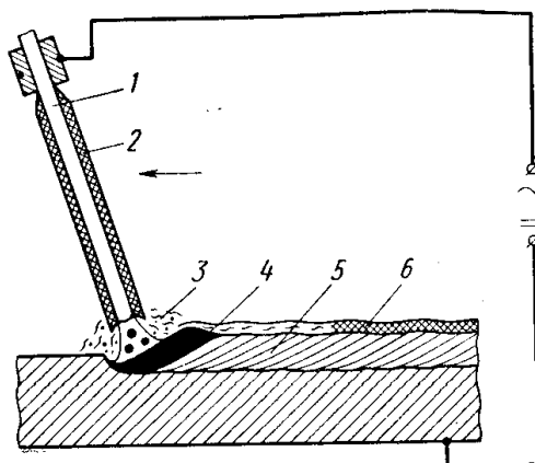
2.1 - rasm. Yoyli dastakli payvandlash chizmasi:
