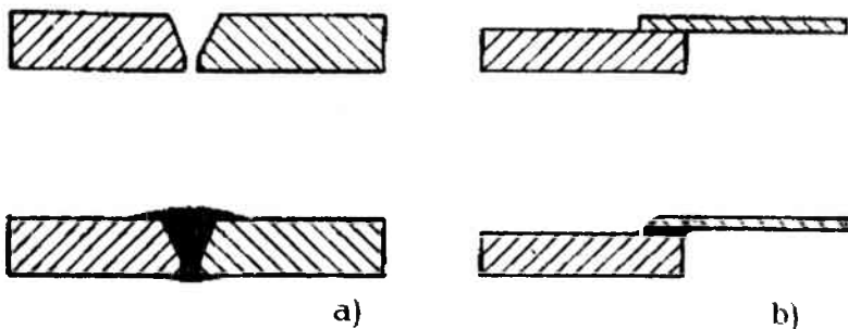
16.4-rasm. Kavsharlash-payvandlashda chok hosil bo'lish sxemasi:
