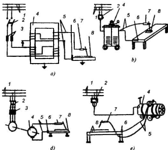
2.2-rasm. Yoy bilan dastakli payvandlash postining sxemasi:
