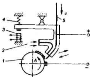
14.3-rasm. Vibro-yoy bilan eritib qoplash:
