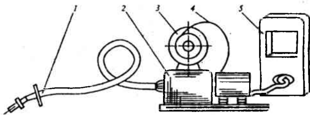
4.4-rasm. Shlangli yarim avtomat chizmasi:
