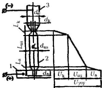
5.1-rasm. Elektr yoyida kuchlanish tushishining taqsimlanish chizmasi: 1 – buyum, 2 – yoy ustuni, 3 – elektrod.
