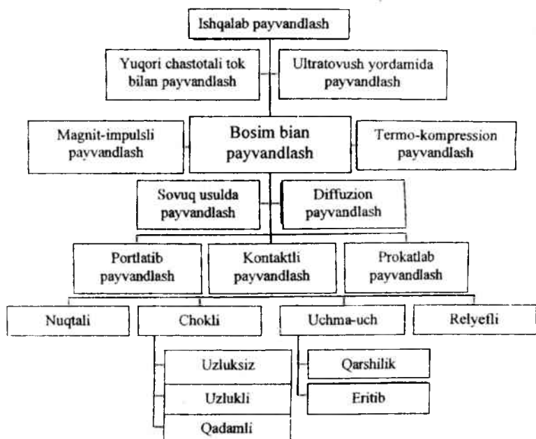
1.6-rasm. Bosim bilan payvandlash usullarining tasnifi.
