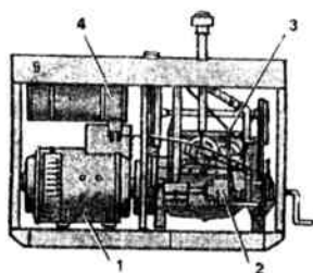
5.9 - rasm. Payvandlash agregati:
