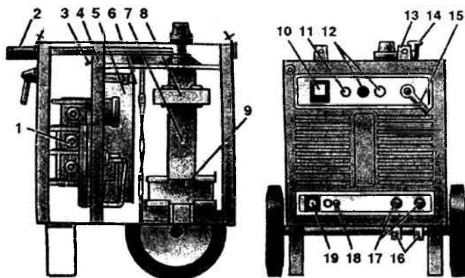
5.7-rasm. Payvandlash to'g'rilagichi:
