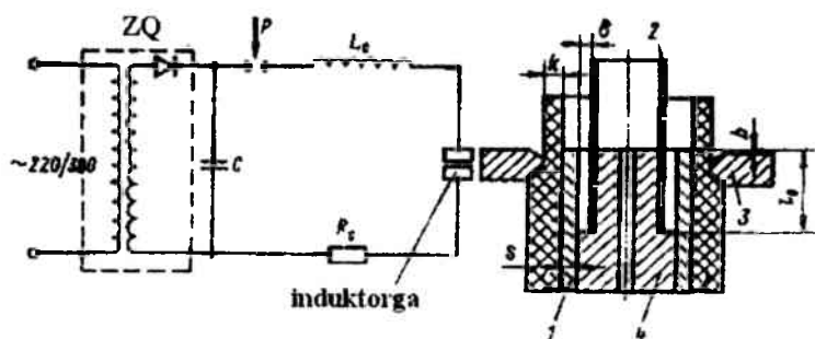
13.3-rasm. Magnit-impulsli payvandlash sxemasi:
