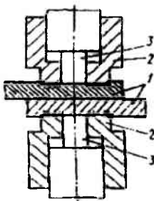
10.2-rasm. Payvandlanayotgan detallarni oldindan qisib bajariladigan sovuq holatda nuqtali payvandlash chizmasi.
