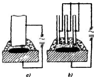
14.2-rasm. Flyus ostida yoy bilan eritib qoplash:
