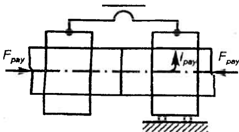
9.4-rasm. Uchma-uch payvandlash sxemasi.
