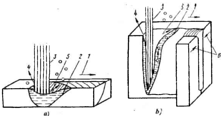
7.2-rasm. Elektron nurli payvandlashning sxematik ko'rinishi:
