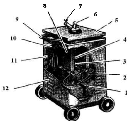
5.3-rasm. Yoy bilan dastakli payvandlash uchun chulg'amli suriladigan transformator:
