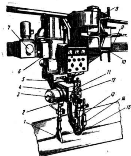
3.2 - rasm. Elektr yoyli flyus ostida payvandlash uchun avtomat:
