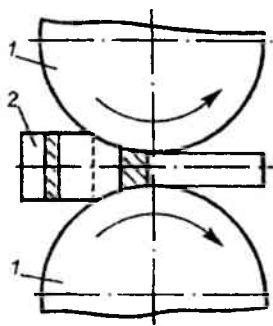
12.4-rasm. Prokatlab payvandlash sxemasi:
