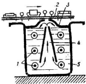
16.8-rasm. Eritilgan kavshar to'liqini bilan kavsharlashning prinsipial sxemasi:
