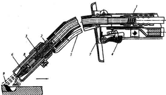
4.5-rasm. A-1197 shlangli yarim avtomat gorelkasi chizmasi:
