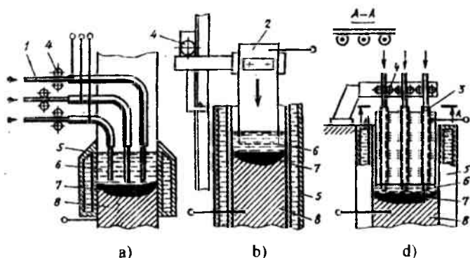
6.2-rasm. Elektr-shlak payvandlash usullari:
