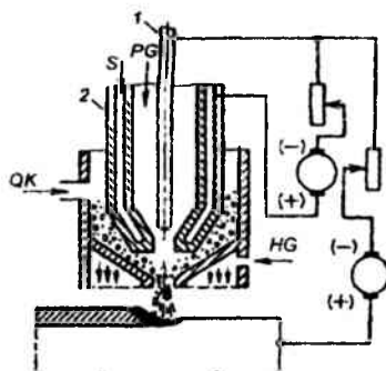
14.6-rasm. Plazma-kukunli eritib qoplash:
