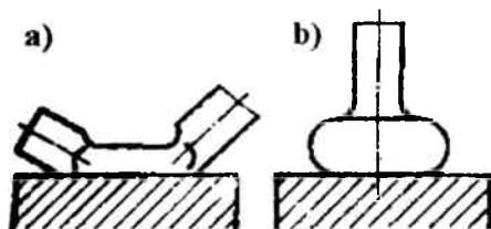
12.2-rasm. Birikma bajarish usuli bo'yicha termokompression payvandlash usullari:
