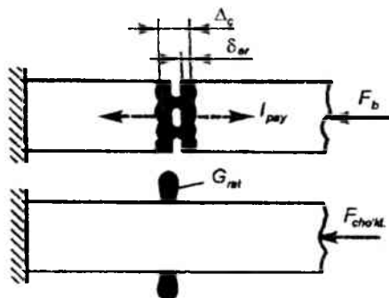
9.6-rasm. Eritib uchma-uch payvandlashda birikma hosil bo'lish sxemasi ( F_b – boshlangich kuch; F_{cho'kt} – cho'ktirish kuchi; \delta_{er} – erigan metall qatlami).
