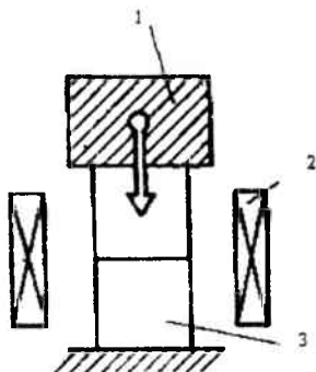
10.4-rasm. Erkin deformatsiyalash sxemasi bo'yicha diffuzion payvandlash:
