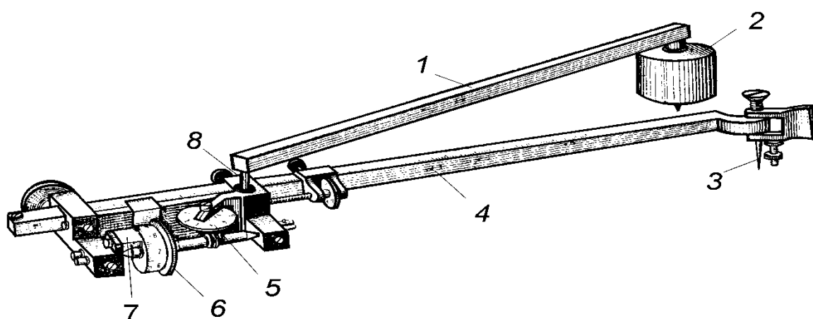
14-rasm. Qutbiy planimetr
