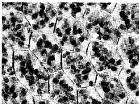
16-rasm. Eukariotlar 11
