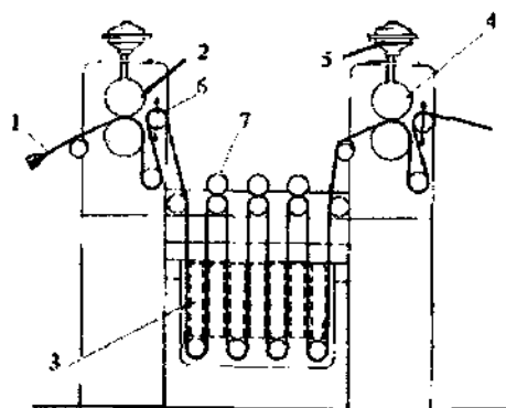
58- rasm. Siqish vallari bor yuvish mashinasi:
