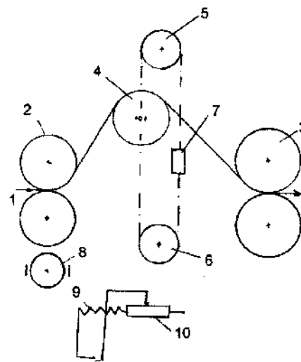
23- rasm. Rolikli taranglovchi datchik sxemasi:
