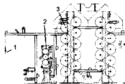
154- rasm. Quritish agregatining sxemasi:
