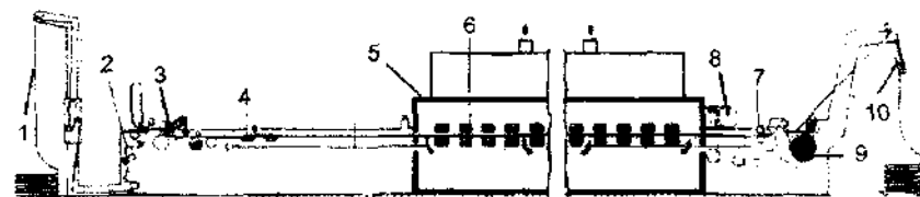
179 – rasm. Quritish-kengaytirish mashinasining sxemasi:
