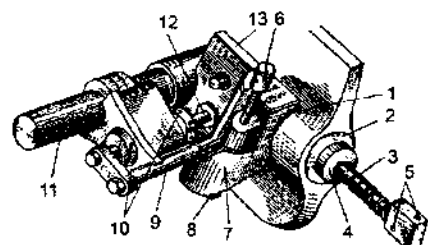
201- rasm. Gul bosish valining mashina gardishiga mahkamlash mexanizmi:
