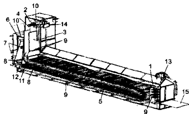
43- rasm. "Vakayama" firmasining ikki yarusli bug'lash kamerasi:
