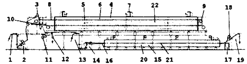
190- rasm. "Vakayama" yakuniy ishlov beruvchi agregatining sxemasi:
