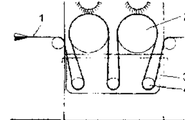
75- rasm. "Menzel" firmasining yuvish-tozalash mashinasidan mato o'tish sxemasi:
