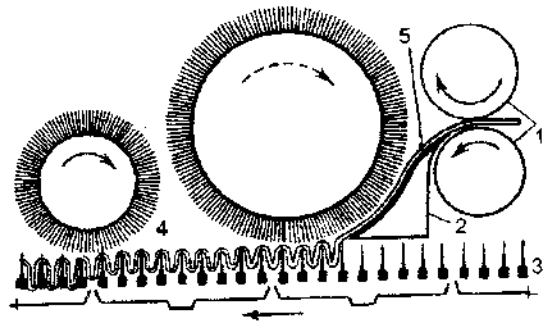
189- rasm. Mato chetini klupp ignalariga sanchish mexanizmining sxemasi:
