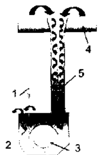
67- rasm. Matoni tor tirqishdan o'tishda yuvish sxemasi:
