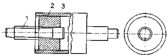
11- rasm. Oddiy yo'naltiruvchi val:
