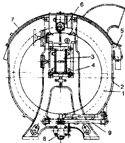
139- rasm. KB – 50 – 1 bo'yash barabanining sxemasi:
