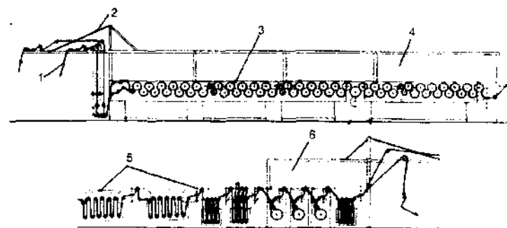
87- rasm. "Vakayama" firmasining zanjirsiz mersevlash agregati sxemasi:
