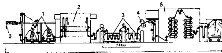
142- rasm. LKZ – 120 bo'yash agregatining sxemasi:
