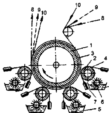
195- rasm. To‘rt valli gul bosish mashinasining sxemasi:
