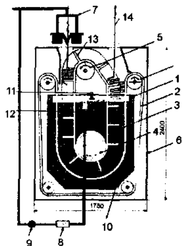
70- rasm. "Hi – Lax" yuvish mashinasining texnologik sxemasi:
