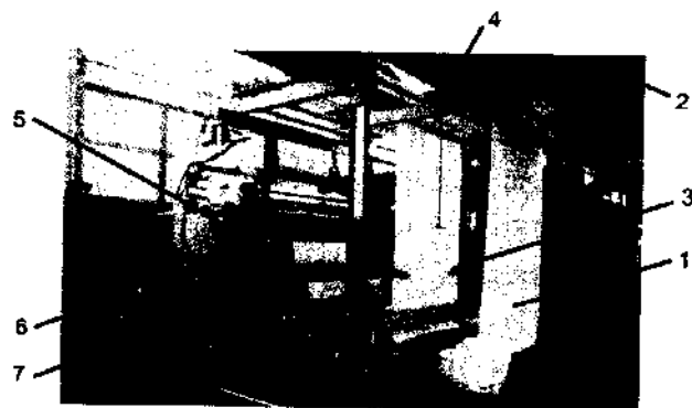
13- rasm. "Vakayama" firmasining uch valli kalandri:
