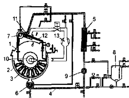
130-rasm. "Then Airflow, AFE" ejektor bo'yash mashinasining texnologik sxemasi
