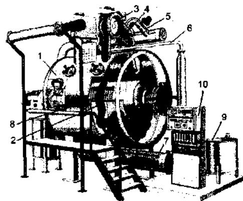
131-rasm. "Then Airflow, AFE" ejektor bo'yash mashinasining kesimi:
