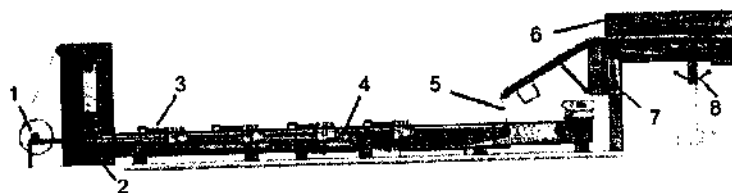
209- rasm. Yassi andozali gul bosish mashinasining sxemasi:
