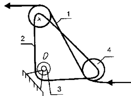
5- rasm. Bremzaning sxemasi: 1 – mato; 2 – bremza gardishi; 3 – aylanish o'qi; 4 – rolik.
