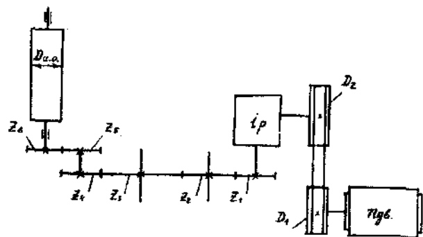
25- rasm. Valli gul bosish mashinasi yurituvchisining kinematik sxemasi
