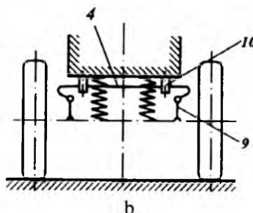
Figure 4.4. The scheme of suspension and antiroll bar.
