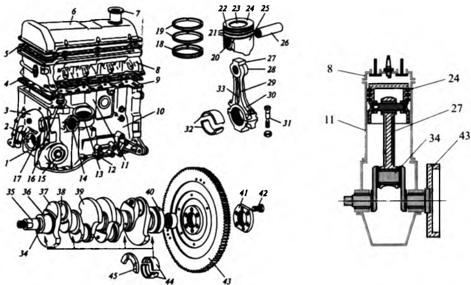
2.5-rasm. Yengil avtomobil dvigateling krivoship-shatunli mexanizmi:
