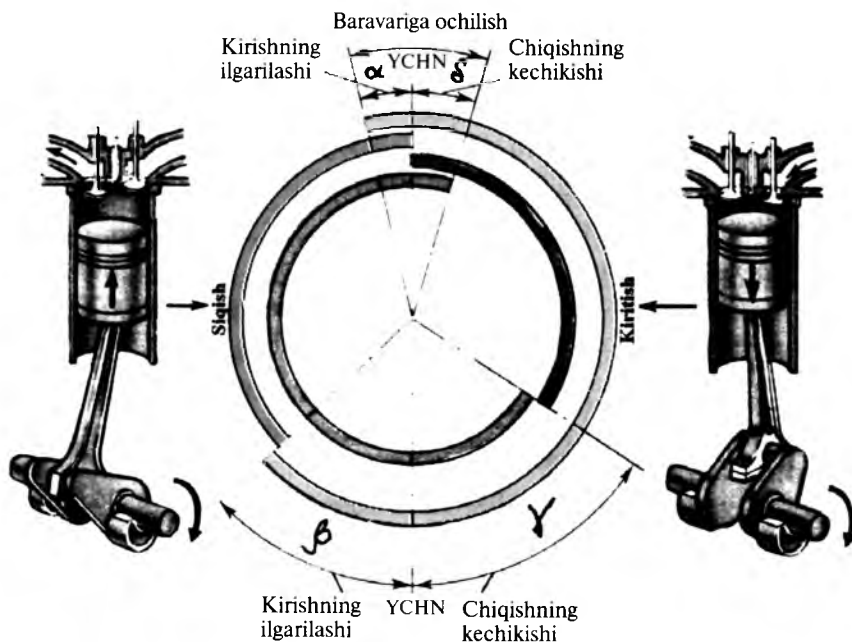
2.7-rasm. Gaz taqsimlash fazasining diagrammasi.
