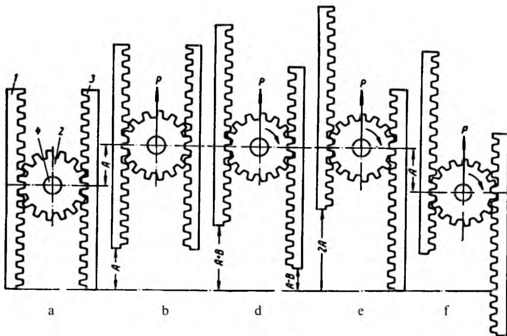
3.20-rasm. Differentialning ishlash sxemasi.
