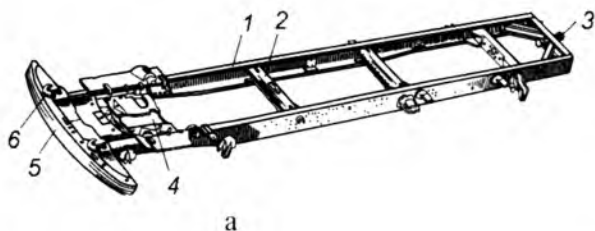
4.8-rasm. Avtomobil ramasi:
