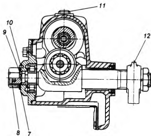
5.11-rasm. Globoidli chervyak va uch o'rkachli rolik rul mexanizmi.
