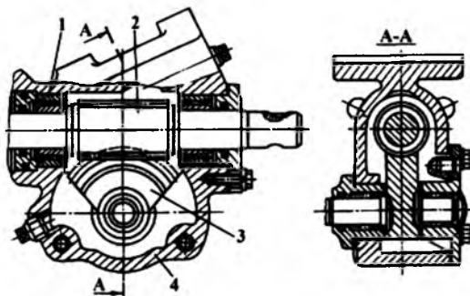
Figure 5.9. Cylinder worm- cylinder spiral toothed wheel.
