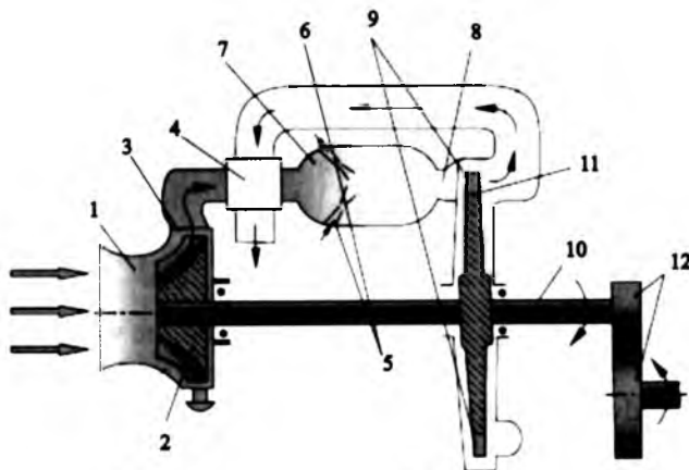
Figure 2.4. The scheme of gas-turbine engine.
