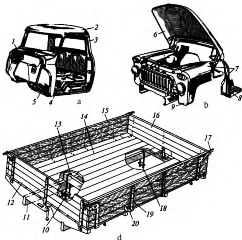
4.11-rasm. Yuk avtomobilining kabina va bort platformali kuzovi.
