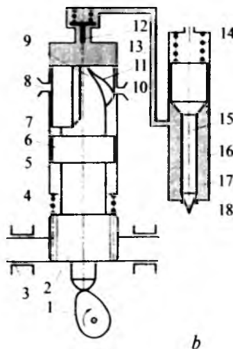
Figure 2.17. Fuel feed scheme from HPFP to cylinder.
