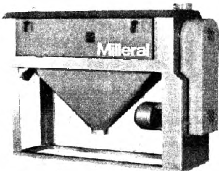
51-rasm. Don yuzasini tozalash uchun gorizontaal ishlov beruvchi mashina
