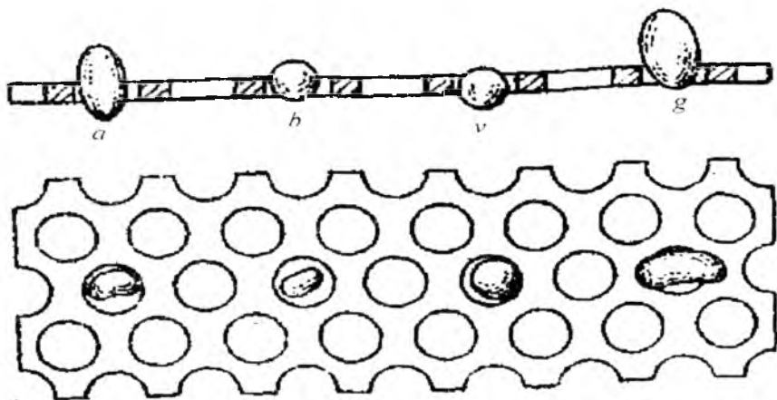
47-rasm. Dumaloq teshikli elaklarda donni chiqindilardan ajratish.
