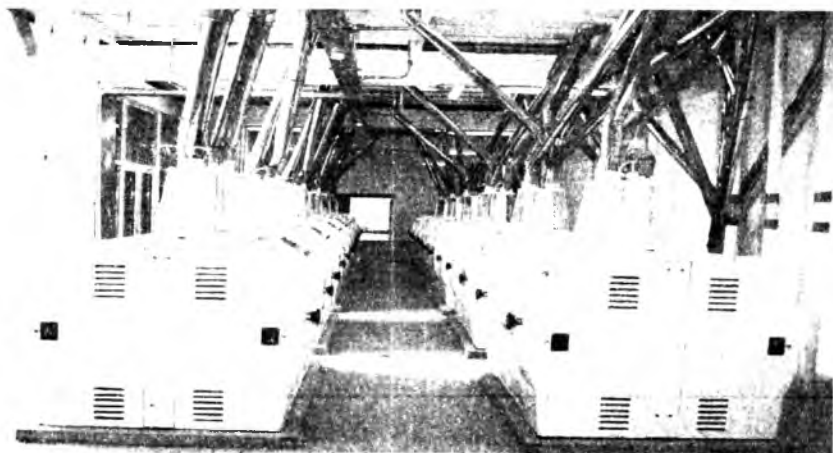
58-rasm. Yanchish bo'limi
