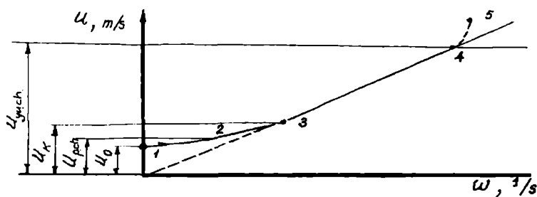
2.17-rasm. Vertushkaning darajalanish (graduirovka) grafigi
