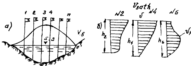
2.11-rasm. Ochiq havzada tezliklarning taqsimlanishi
