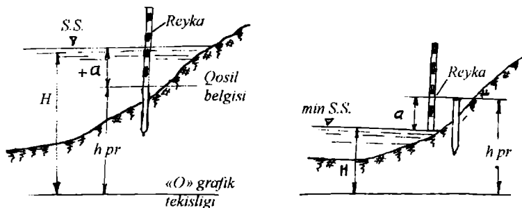
2.3-rasm. Suv sathini nol grafikka nisbatan o'lchash
