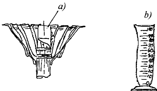
1.4-rasm V.D.Tretyakov yog'in o'lchagichi:
