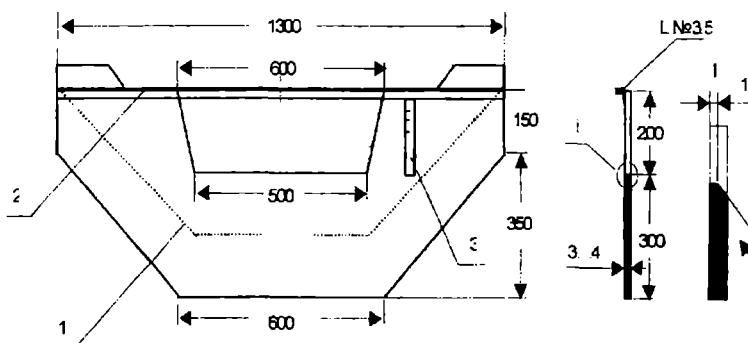
2.33-rasm. Trapetsiya shaklidagi Chipoletti (VCh-50) suv o‘lchagichi: (vodoslivi), tubining kengligi 500 mm (50 sm, 1 sm-10 mm)
