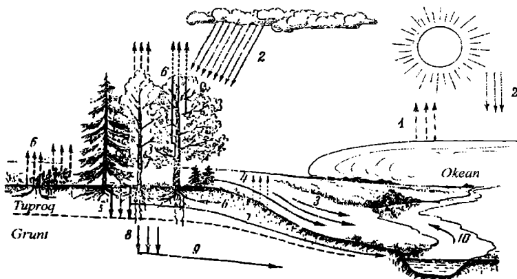
1.1-rasm. Tabiatda suvning aylanishi
