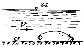
2.31-rasm. Suv osti oqizqlar harakati
