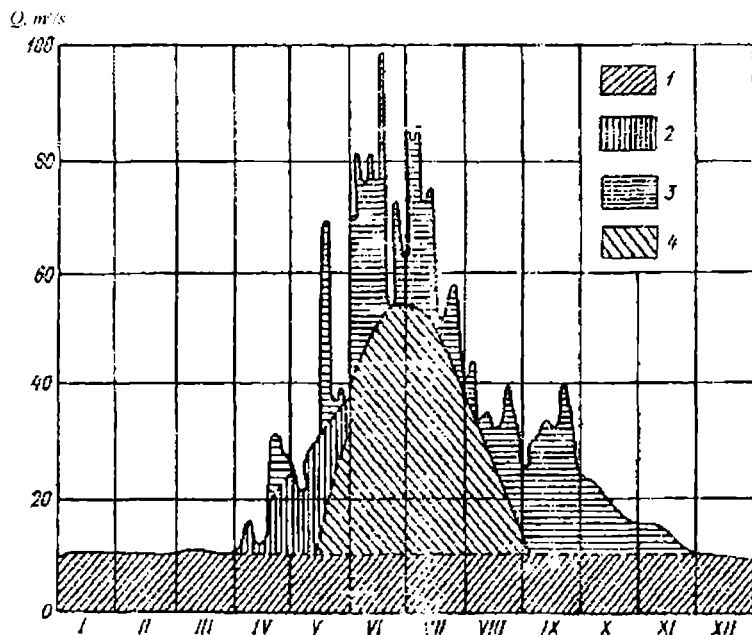
1.11-rasm. Tog' daryosi gidrografini ajratish
