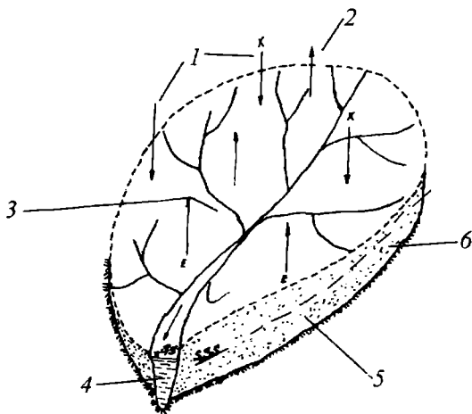
1.2-rasm. Daryo havzasining suv balansi chizmasi
