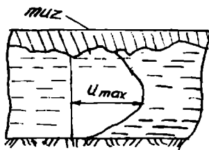
2.12(b)-rasm. Muz ostidagi tezlik
