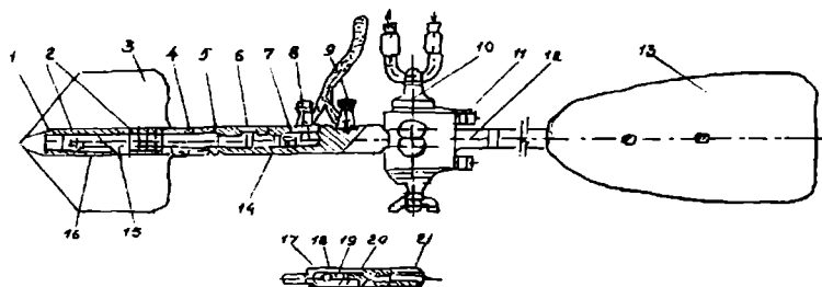
2.16-rasm. Vertushka GR-21M ning tuzilishi
