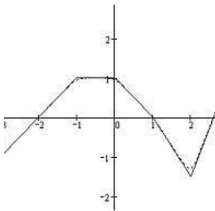
Figure 1.1: A piecewise linear function on [-3, 3] .
