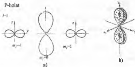
17.8-rasm. a) \theta - burchakka bog'liq bo'lgan p_\theta = |\theta'|^2 va
