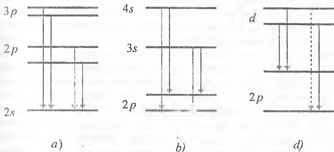
18.10-rasm. a)- p sathlardan 2s sathga o'tish chizmasi;
