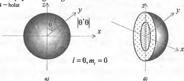
17.7-rasm. a) \theta - burchakka bog'liq bo'lgan p_\theta = |\theta'|^2
