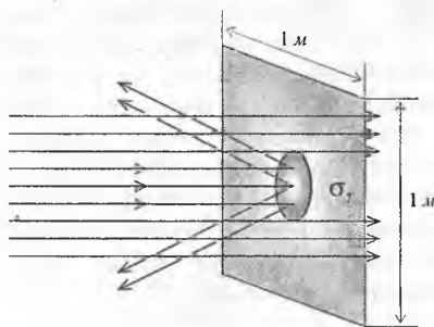
20.6- pacm. Sochilishning Tompson kesimi ( \sigma_T ).
