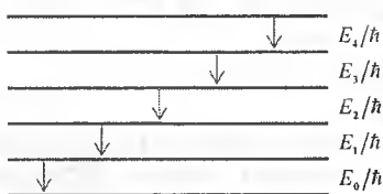
20.8-рasm. Garmonik ossillator uchun ruxsat etilgan o'tishlar
