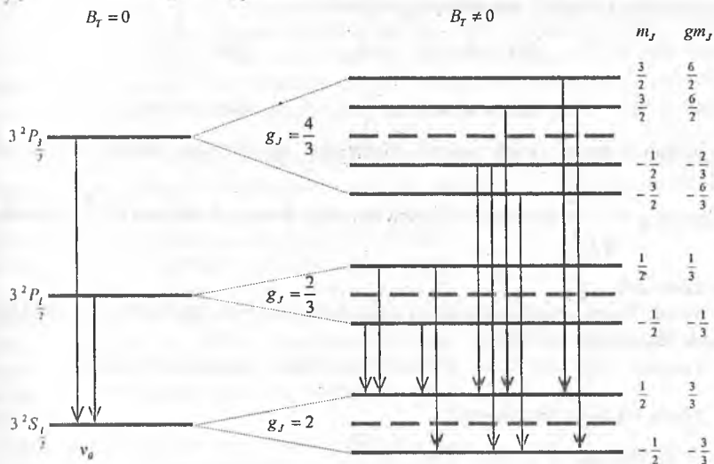
19.4-рasm. Atom sathlarining kuchsiz magnit maydonda Zeyeman anomal ajralishi
