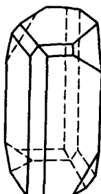
\beta - S
