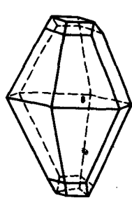
\alpha - S
