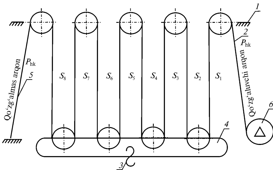
6-rasm. 4 \times 5 osnastka:
