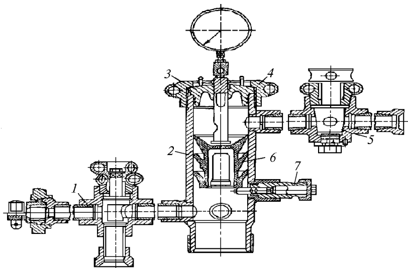
39-rasm. Quduq og'zini sementlash kallagi 2ГΥΠ-400.
