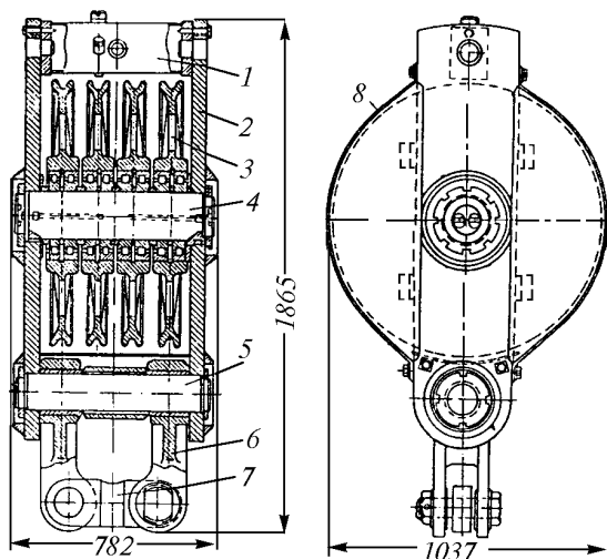
8-rasm. TBH4-75 tal bloki:
