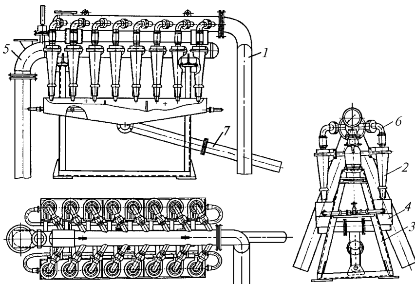
20-rasm. ПГ—45 chang tozalagich:
