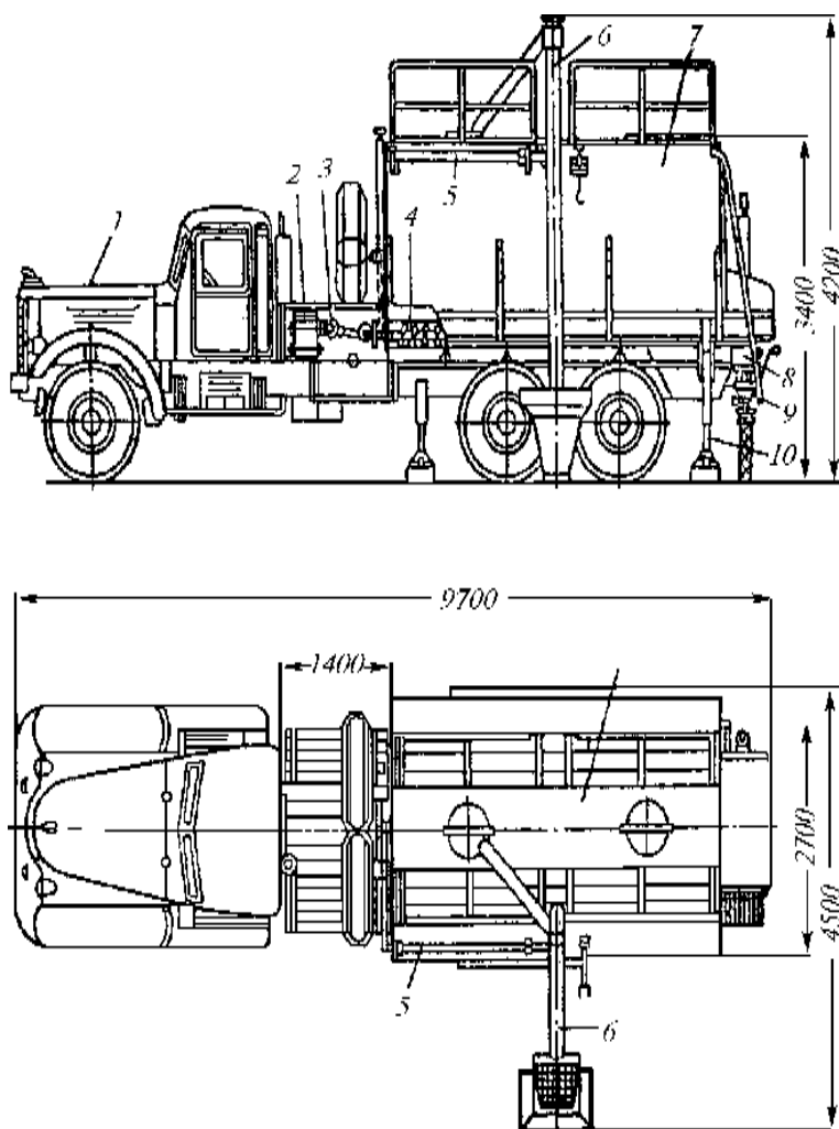
38-rasm. Sement qorishtirgich mashinasi — 2CMH-20:
