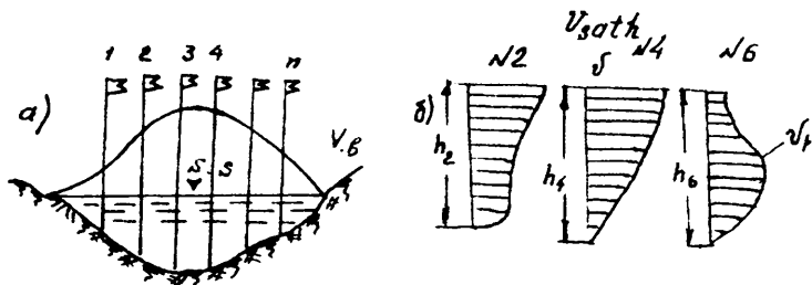
2.11-rasm. Ochiq havzada tezliklarning taqsimlanishi
