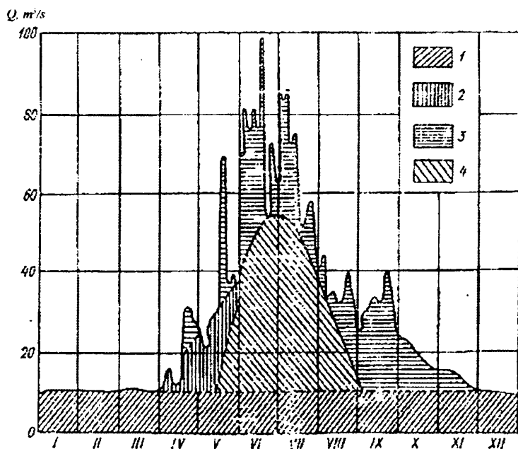
1.11-rasm. Tog' daryosi gidrografini ajratish
