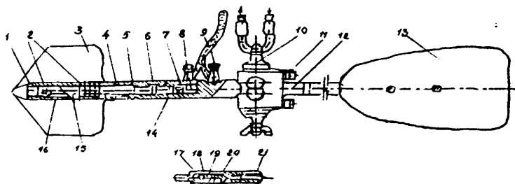
2.16-rasm. Vertushka GR-21M ning tuzilishi
