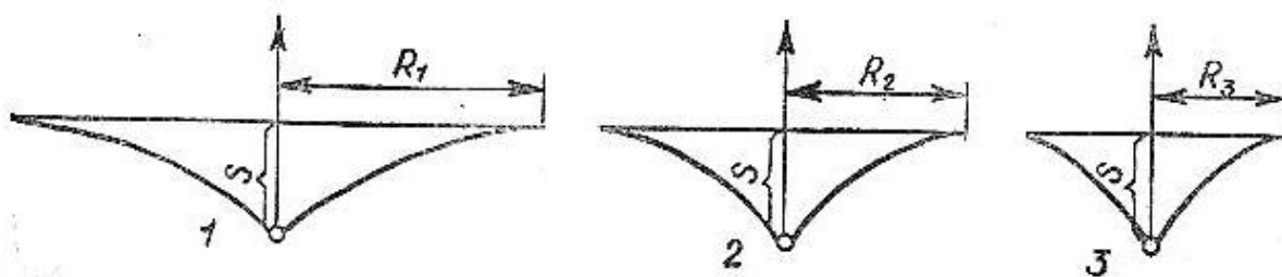
16.9 - rasm. Deprssion voronkalar; 1 – shag'al; 2 – qum; 3 – qumotuproq
