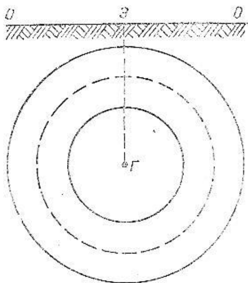
13.1 – rasm. Zilzilaning gipotsentri va epitsentri: G –giposentr; E –episentr
