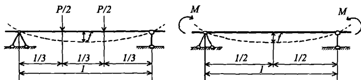
66-rasm. Yog‘ochning deformatsiyalanishi.
