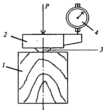
67-rasm. Yog'och tanasining statik qattiqligini sinash shakli:
